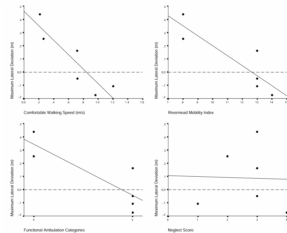
Figure 2. Scatterplots of Maximum Lateral Deviation (MLD) vs. Comfortable Walking Speed, Rivermead Mobility Index (RMI), Functional Ambulation Categories (FAC) and Neglect Score for right hemisphere stroke patients with neglect.
