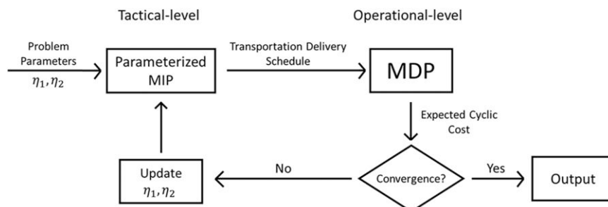
Figure 3. The Framework of Our Approach
