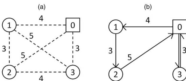
Figure A.1. Locations (a) and the Associated Routing (b) for the Illustrative SCIRP Example
