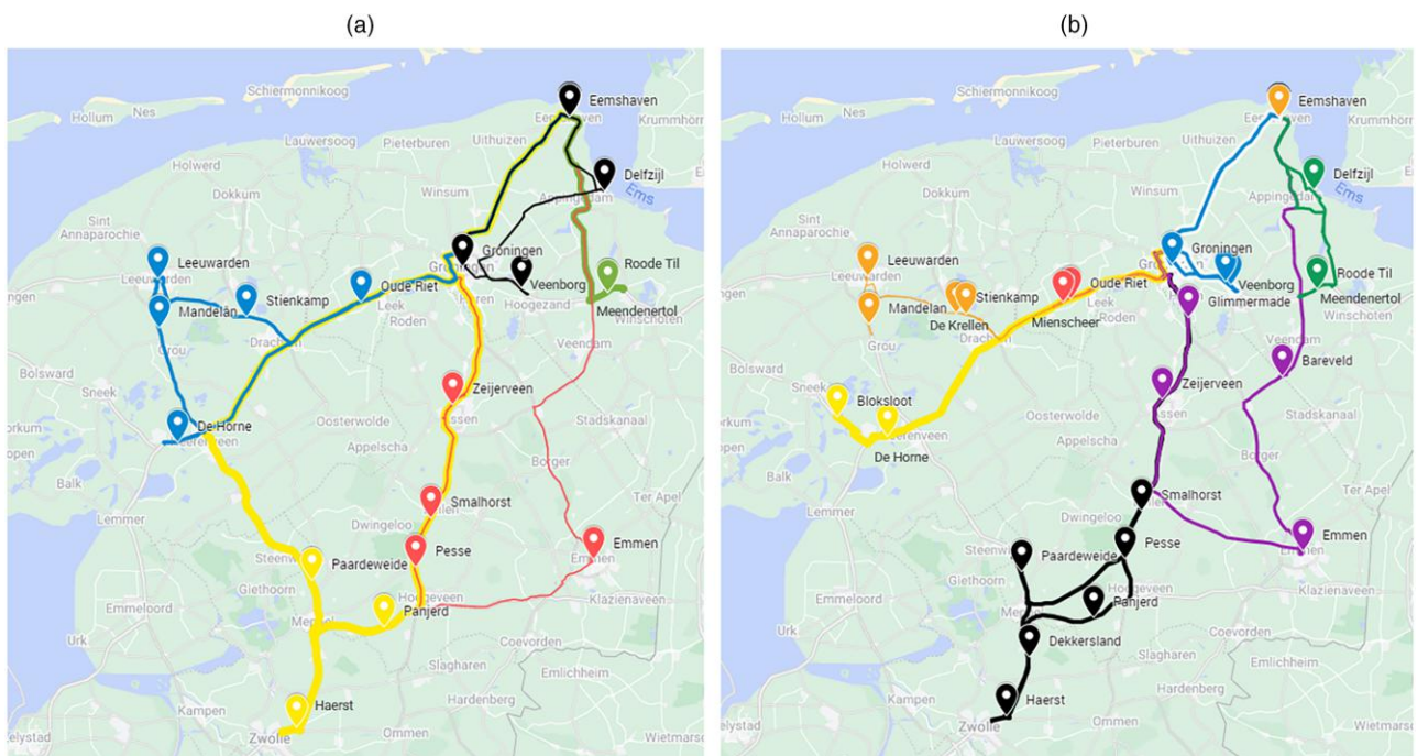
Figure 7. (Color online) The Routing on Eemshaven Cases in the Suggested Policy
