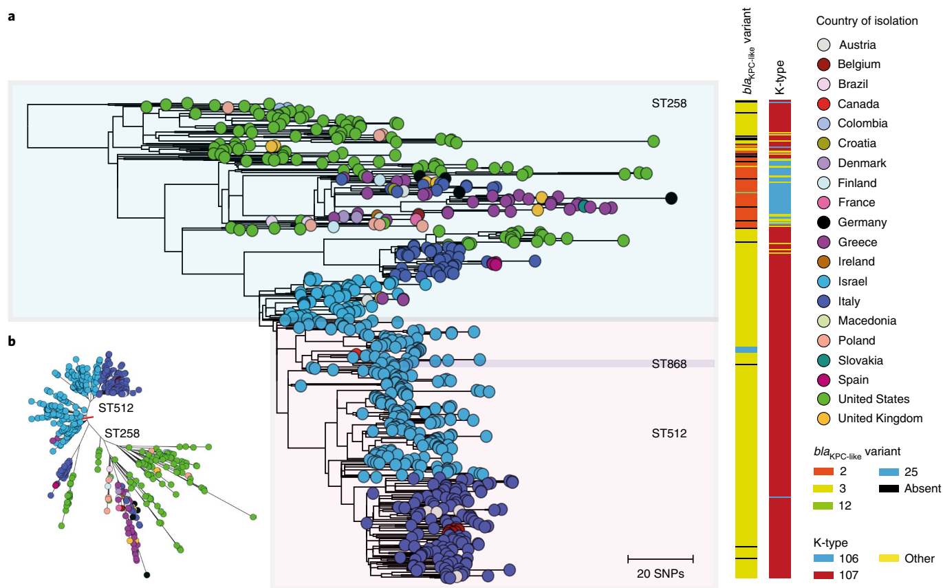
Fig. 5 | International spread of the epidemic ST258/512 clone. a , A phylogenetic tree of 651 isolates of ST258 and 512 (and a derivative of ST512, ST868), comprising 236 isolates submitted during the EuSCAPE survey and 415 isolates with publicly available sequence data. The tree was rooted using an ST11 isolate that was later removed. The colours of the isolate tips represent the country of isolation and metadata columns show the bla KPC-like variant and K-type. b , An unrooted version of the tree shown in a . Similar visualizations are available at: https://microreact.org/project/EuSCAPE_ST258/bbafcc1c ( a ) and https://microreact.org/project/EuSCAPE_ST258/dd960284 ( b ).
