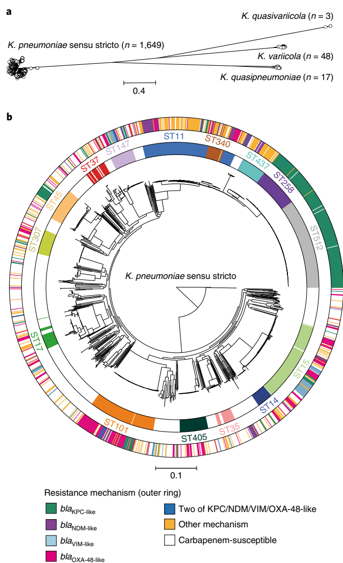
Fig. 2 | Carbapenemase-positive isolates are concentrated in major clonal lineages of K. pneumoniae . a , A phylogenetic tree of the 1,717 EuSCAPE isolates analysed in this study (constructed using 2,539 core genes) demonstrating the division into four species. b , A phylogenetic tree of 1,649 isolates belonging to K. pneumoniae sensu stricto ; STs containing more than 20 isolates are shown in the inner ring and labelled. In the outer ring, isolates are coloured by resistance mechanism as in Fig. 1a. The scale in both trees represents the number of single nucleotide polymorphisms (SNPs) per variable site. Similar visualizations are available at: https://microreact.org/project/EuSCAPE_Kp/bc81fffe ( a ) and https://microreact.org/project/EuSCAPE_Kp/2585de34 ( b ).
