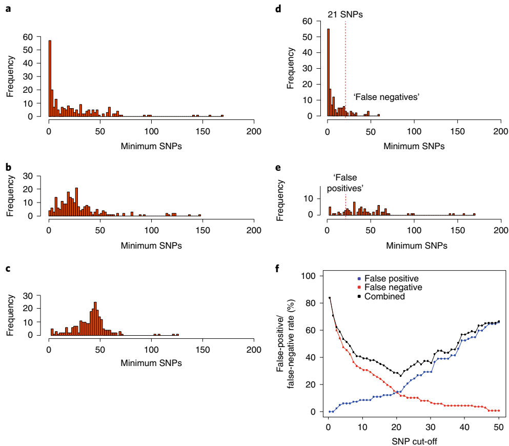
Fig. 4 | Determination of a SNP cut-off to aid outbreak investigations of ST258/512. a–c , The number of core chromosomal SNPs between each of the 236 ST258/512 isolates submitted during EuSCAPE and the most closely related isolate submitted by the same hospital ( a ), a different hospital in the same country ( b ) and a hospital in a different country ( c ). d,e , The number of SNPs between each ST258/512 isolate and the most closely related isolate submitted by the same hospital, when isolates are predicted to have been involved in intrahospital ( d ) or interhospital ( e ) transmission. The dotted lines are drawn at the number of SNPs at which the combined false-positive and false-negative rates for correctly identifying intrahospital transmission, calculated using the predictions as the reference, are at a minimum. f , False-positive and false-negative rates when different SNP cut-offs are used.
