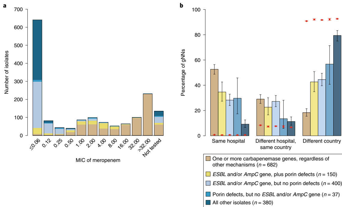
Fig. 3 | Carbapenemase-positive isolates show strong geographical clustering. a , Bar plots showing the distribution of MIC values among 1,518 retested K. pneumoniae sensu stricto isolates with different \beta -lactam resistance determinants. b , Bar plots showing the proportions of gNNs for K. pneumoniae sensu stricto isolates with different \beta -lactam resistance determinants that are from different geographic contexts (the same hospital, a different hospital in the same country, or a hospital in a different country). The black error bars represent the 95% CIs of these proportions. The proportions of gNNs in the absence of geographic structure were calculated from 100 repeat analyses in which the hospital codes were randomly permuted; the means and 95% CIs of these results are shown in red.
