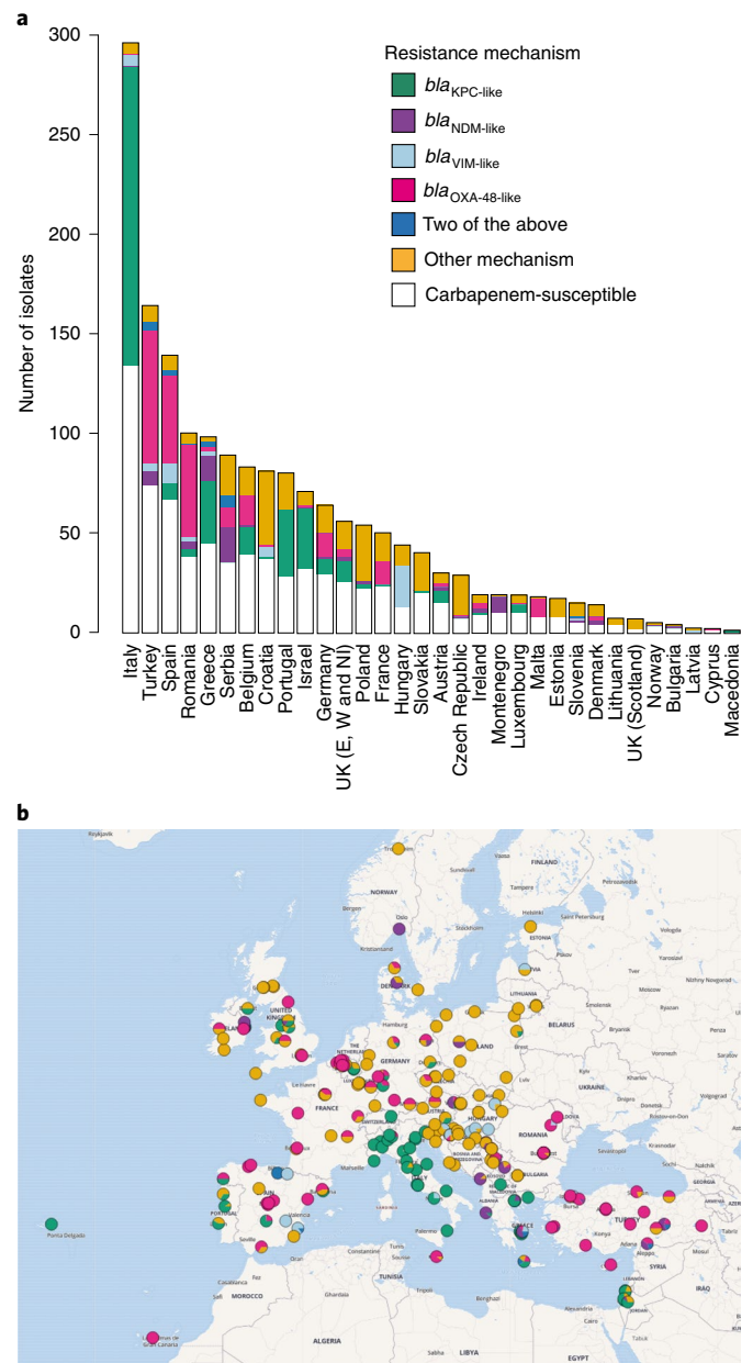
Fig. 1 | Geographical distribution of carbapenem resistance mechanisms among isolates submitted during the EuSCAPE survey. a , All of the isolates submitted by participating countries and analysed in this study, partitioned into: those that possess one or more of four major carbapenemase genes ( bla KPC-like , bla OXA-48-like , bla NDM-like and bla VIM-like ), regardless of whether they were submitted as carbapenem-non-susceptible or -susceptible; those that lack any of the four genes and were submitted as carbapenem-non-susceptible ('Other mechanism'); and those submitted as carbapenem-susceptible. b , Pie charts showing the proportions of different resistance mechanisms in isolates submitted as carbapenem-non-susceptible by participating hospitals. Colour key as in a . E, England; W, Wales; NI, Northern Ireland.
