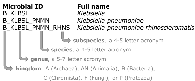
Figure 1: The structure of a typical microbial ID as used in the AMR package. An ID consists of two to four elements, separated by an underscore. The first element is the abbreviation of the taxonomic kingdom. The remaining elements consist of abbreviations of the lowest taxonomic levels of every microorganism: genus, species (if available) and subspecies (if available). Abbreviations used for the microbial IDs of microorganism names were created using the base R function abbreviate() .
