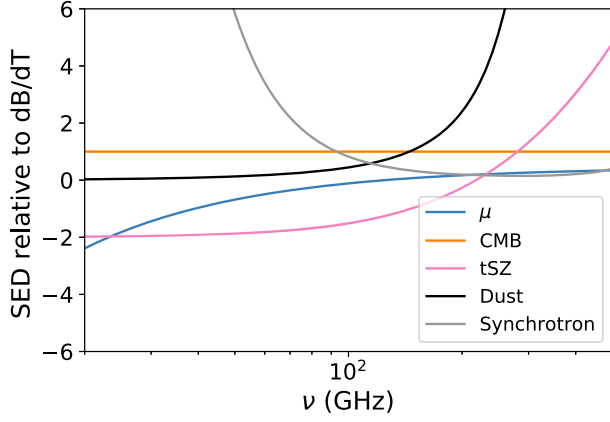
FIG. 2. Spectral shape of CMB anisotropy, \mu distortions, and various Galactic and extragalactic foregrounds, all divided by the CMB anisotropy SED and scaled by an arbitrary amplitude. For frequencies \nu < 100 GHz, we see that Galactic synchrotron sharply rises, even relative to \mu distortions. At frequencies \nu > 100 GHz, Galactic dust and the thermal SZ effect start growing as the \mu -distortion spectrum starts leveling off.
