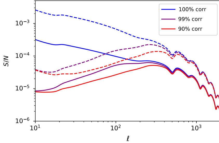
FIG. 5. S/N per multipole for various assumed values of atmospheric correlation between bands. Dashed lines correspond to S/N when only including instrumental and atmospheric noise, while solid lines also include the effects of foregrounds. In all cases, the y SED has been projected out (see text for details).
