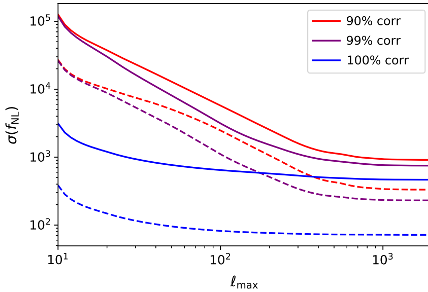
FIG. 6. 1\sigma constraints on f_{\text{NL}} as a function of the maximum multipole used in analysis, \ell_{\text{max}} . Dashed lines correspond to \sigma(f_{\text{NL}}) when only including instrumental and atmospheric noise, while solid lines also include the effects of foregrounds. In all cases, the y SED has been projected out (see text for details).
