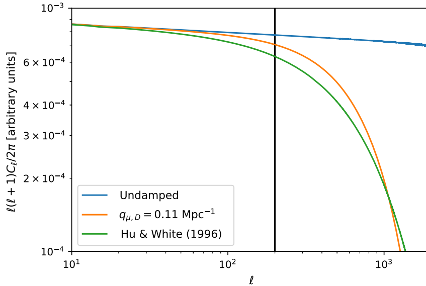
FIG. 7. Change in the angular power spectrum C_\ell depending on the damping factor. For illustrative purposes, we choose an undamped spectrum that is nearly scale invariant, with a slight spectral tilt. The spectrum with a damping scale q_{\mu,D} = 0.11 \text{ Mpc}^{-1} corresponds to our treatment of the damping of \mu anisotropies. The spectrum using the damping factor from Ref. [58] has more severe damping at \ell = 200 , but has a slightly less steep slope compared to the \mu -anisotropy damping scale. The black line corresponding to \ell = 200 is a reference scale for the reader.
