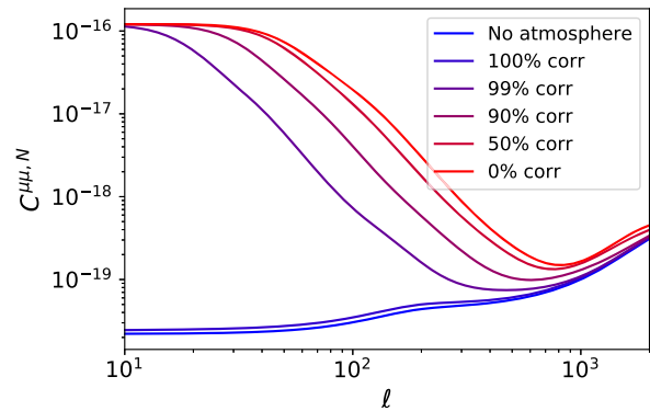
FIG. 4. C_{\ell}^{\mu,N} for the CMB-S4 ultra-deep survey and various assumptions for the degree of atmospheric correlation between bands. Full correlation among bands closely matches the nominal case of no atmosphere. However, even minimal decorrelation among detectors significantly worsens C_{\ell}^{\mu,N} at low multipoles.
