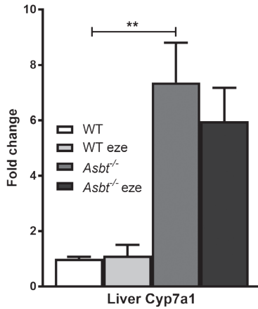
Supplemental Figure S1: Hepatic Cyp7a1 expression in WT and Asbt -/- mice with and without ezetimibe treatment; n=5-6 per group.
