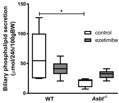
Supplemental Figure S5: Biliary phospholipid secretion in WT and Asbt -/- mice with and without ezetimibe treatment; n=5-6 per group.
