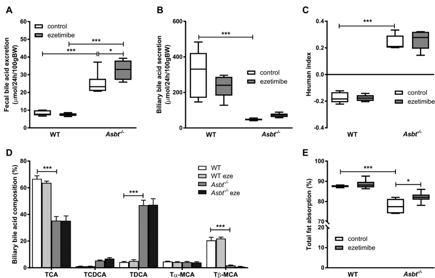
Figure 4: Changes in fecal and biliary bile acids and intestinal fat absorption upon ezetimibe treatment and Asbt deletion in mice. Total fecal bile acid excretion (A) , total biliary bile acids secretion (B) , biliary hydrophobicity index based on Heuman values (C) , biliary bile acid composition (D) and intestinal fatty acid absorption (E) ; n=5-6 per group.
