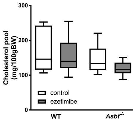
Supplemental Figure S4: Whole body cholesterol pool in WT and Asbt -/- mice with and without ezetimibe treatment; n=5-6 per group.
