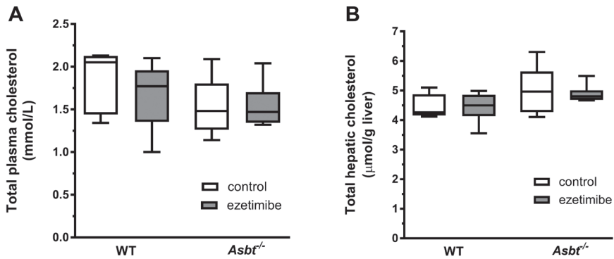
Supplemental Figure S2: Total plasma and hepatic cholesterol concentrations in WT and Asbt -/- mice with and without ezetimibe treatment. Total plasma cholesterol (A) and total liver cholesterol content (B); n=5-6 per group.
