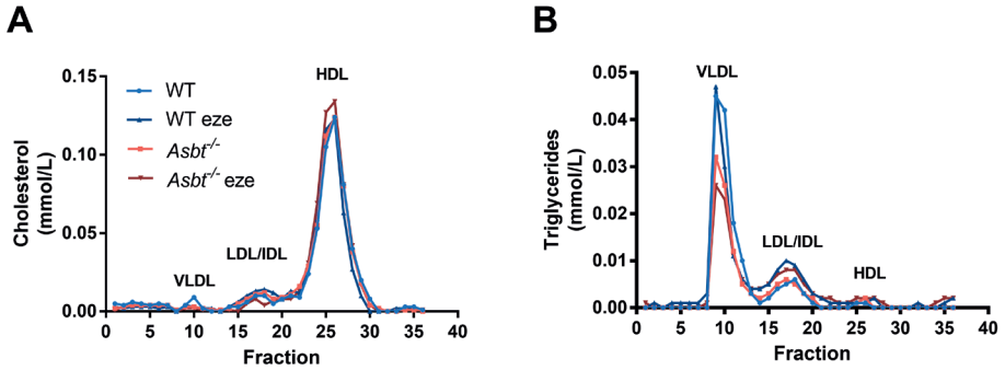
Supplemental Figure S3: Pooled plasma lipoprotein fractions separated by fast performance liquid chromatography (FPLC). Measured for cholesterol ( A ) and triglycerides ( B ); n=5-6 pooled samples per group.
