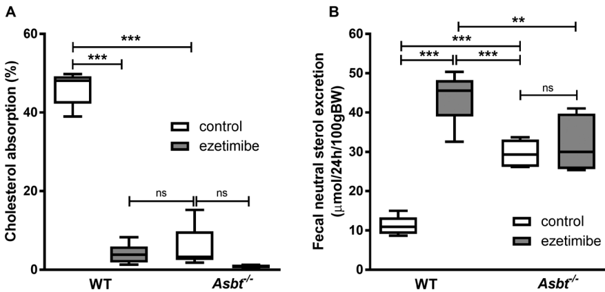
Figure 2: Intestinal cholesterol absorption and fecal neutral sterol excretion in WT and Asbt -/- mice with and without ezetimibe treatment. Fractional cholesterol absorption ( A ) measured by stable dual isotope method. Total neutral sterol excretion in feces ( B ); n=5-6 per group.
