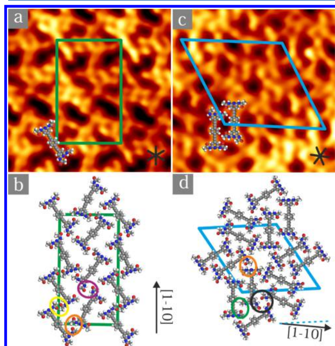
Figure 2. Comparison of the molecular arrangements \alpha and \beta . (a) High-resolution STM image of molecular arrangement \alpha ( 8 \times 8 \text{ nm}^2 , 0.1 V, and 170 pA). The black lines indicate the principal directions of the Au(111) substrate. The unit cell is shown in green. A molecular model of 1 is overlaid to guide the eye. (b) Tentative structural model of arrangement \alpha . The long axis of the unit cell aligns with the [1\bar{1}0] direction of the Au(111) substrate. The arrangement is stabilized by different H-bonding interactions (marked by orange, yellow, and magenta circles). (c) High-resolution STM image of molecular arrangement \beta ( 7 \times 7 \text{ nm}^2 , 0.1 V, and 170 pA). The unit cell is shown in cyan. (d) Tentative structural model of arrangement \beta . The arrangement is stabilized by a combination of single (marked by green circles), double (marked by orange circles), and cyclic trimeric H-bonds involving three molecules (marked by a black circle). The unit cell is rotated by \gamma = \pm 8^\circ with respect to the [1\bar{1}0] Au direction.
