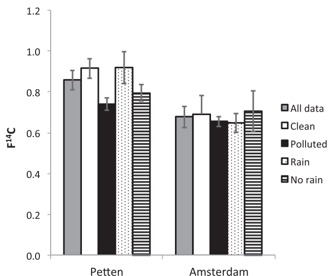
Fig. 2. Averages of F 14 C(OC) in Amsterdam and Petten, for all data, clean and polluted time periods and rainy and dry periods. The error bars refer to the standard error of the mean. If the standard errors do not overlap, the difference between the means is usually considered significant. However with small samples sizes as used here, the standard errors should be considered with caution and be more regarded as a rough indication.
