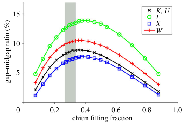
Figure 5. Filling factor dependency of the partial photonic bandgap widths for single diamond photonic crystals. Gap-midgap ratios are shown for the partial bandgaps along the high-symmetry directions K = U, L, W and X . The observed filling fraction for the wing scales of Entimus imperialis is shown in grey; the dielectric constant of the biomaterial chitin was \epsilon = 2.45 . The filling fraction of the weevil scales is on the lower edge of the optimal reflectance plateau, indicating an optimal weight-reflectance ratio.
