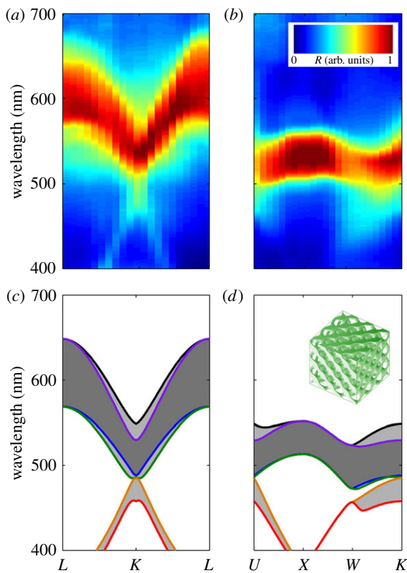
Figure 4. Photonic band structure diagrams (PBSDs). Measured ( a,b ) and simulated ( c,d ) PBSDs for a single-network diamond-type photonic crystal ( Fd\bar{3}m ) along the paths ( a,c ) L-K-L and ( b,d ) U-X-W-K , respectively. The grey areas in ( c,d ) indicate the photonic bandgap of the investigated structure, corresponding to the measured reflectance bands in ( a,b ). In the simulation, the dielectric constant was \epsilon = 2.45 and the chitin filling fraction was approximately 0.3 ( t = -0.5 ). For the wavelength conversion in ( c,d ), the cubic lattice constant of the photonic crystal was set to a = 445 nm (see also electronic supplementary material, figure S4). The inset shows a rendered model of the single diamond photonic crystal.
