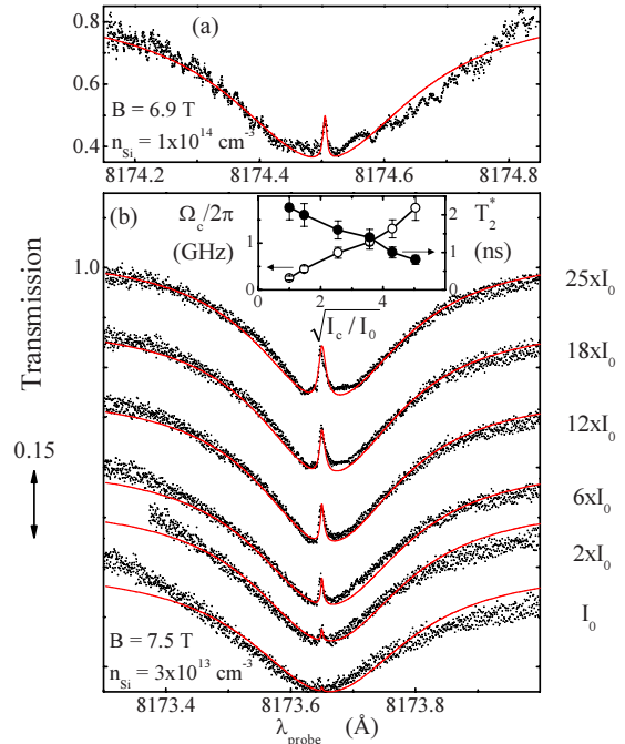
FIG. 2. (Color online) (a) EIT spectrum from sample with Si doping at 1 \times 10^{14} \text{ cm}^{-3} . Dots—experiment. Line—numerical fit. (b) EIT spectra from sample with Si doping at 3 \times 10^{13} \text{ cm}^{-3} , for probe-field intensity 0.04 \text{ W cm}^{-2} and a range of control-field intensities I_c with I_0=0.4 \text{ W cm}^{-2} . The inset shows the fitting results for Rabi frequency \Omega_c and spin dephasing time T_2^* .
