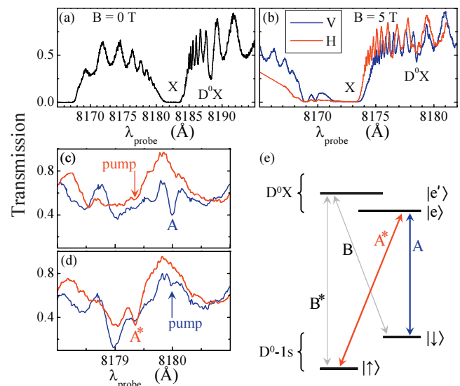
FIG. 1. (Color) (a) Transmission spectroscopy at B=0 T. (b) Transmission at B=5.0 T for H and V polarization. (c) Pump-assisted spectroscopy with H-polarized pumping at the A^* transition shows enhanced absorption for the A transition for the scan with a V-polarized probe (blue trace) but not with an H-polarized probe (red trace). (d) Complementary to (c), V-polarized pumping at A shows enhanced absorption for the A^* transition with an H-polarized probe. (e) Energy levels and optical transitions of the D^0 - D^0X system.
