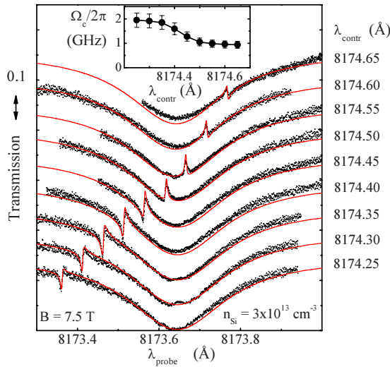
FIG. 3. (Color online) Dependence of EIT spectra on control-field detuning. The position of the EIT peak follows precisely the control-field detuning from transition A. Dots—experiment with control (probe) intensity 6(0.04) W cm ^{-2} . Lines—fits with T_2^* = 2 ns and \Omega_c as presented in the inset.
