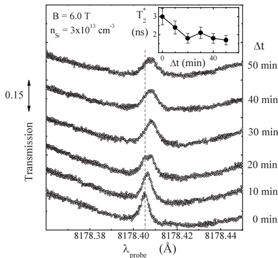
FIG. 4. Evolution of the EIT peak after 30 min pumping of the A^* transition. Fast EIT snapshots were taken at 10 min intervals during which the sample was kept in the dark. The dashed line is a guide for showing the shift in peak position. The inset presents fitting results that show the change in T_2^* .
