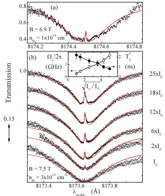
FIG. 2. (Color online) (a) EIT spectrum from sample with Si doping at 1 \times 10^{14} \text{ cm}^{-3} . Dots—experiment. Line—numerical fit. (b) EIT spectra from sample with Si doping at 3 \times 10^{13} \text{ cm}^{-3} , for probe-field intensity 0.04 \text{ W cm}^{-2} and a range of control-field intensities I_c with I_0=0.4 \text{ W cm}^{-2} . The inset shows the fitting results for Rabi frequency \Omega_c and spin dephasing time T_2^* .
