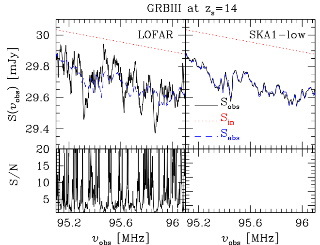
Figure 3. As Fig. 1, but the GRBIII is positioned at z_s = 14 (i.e. \nu \sim 95 MHz) and \Delta\nu = 20 kHz. Note that the S/N in the lower-right panel is always higher than the range covered by the axis.
