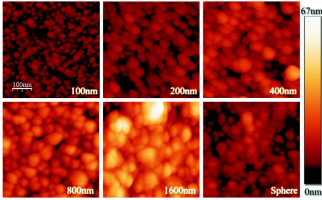
FIG. 1. (Color online) Surface scans of all films and the sphere surface. The scan size is 500 nm and the color range corresponds to indicated range by the color bar.
