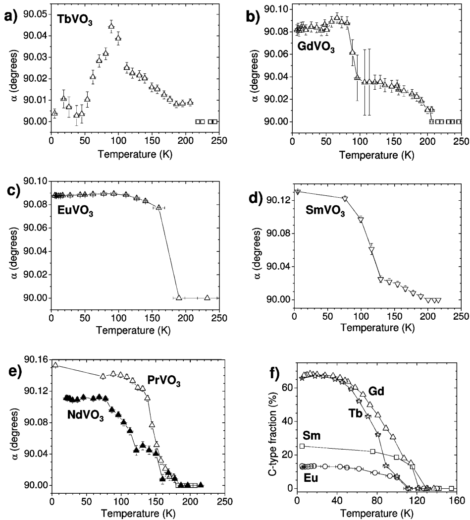
FIG. 4. Temperature dependence of the monoclinic angle, \alpha for (a) \text{TbVO}_3 , (b) \text{GdVO}_3 , (c) \text{EuVO}_3 , (d) \text{SmVO}_3 , (e) \text{NdVO}_3 , and \text{PrVO}_3 . (f) Temperature dependence of the fraction of the C-type OO phase for R\text{VO}_3 ( R = \text{Tb, Gd, Eu, Sm} ).
