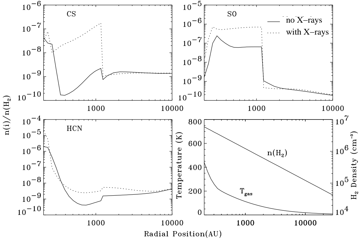
Fig. 4. a - c: Radial models of chemical abundance as derived by Stauber et al. (2005). The solid curve shows the model of the envelope without far-UV and X-ray irradiation by the central object (no-X model), and the dotted curve shows the X-ray model including an X-ray luminosity of 8 \cdot 10^{31} erg s ^{-1} and protostellar far-UV irradiation of G_0 = 10 at 200 AU fitting best to the single-dish data on 24 molecules. Fig. 4d: Density and temperature model of AFGL 2591 used for chemical modeling (see text).
