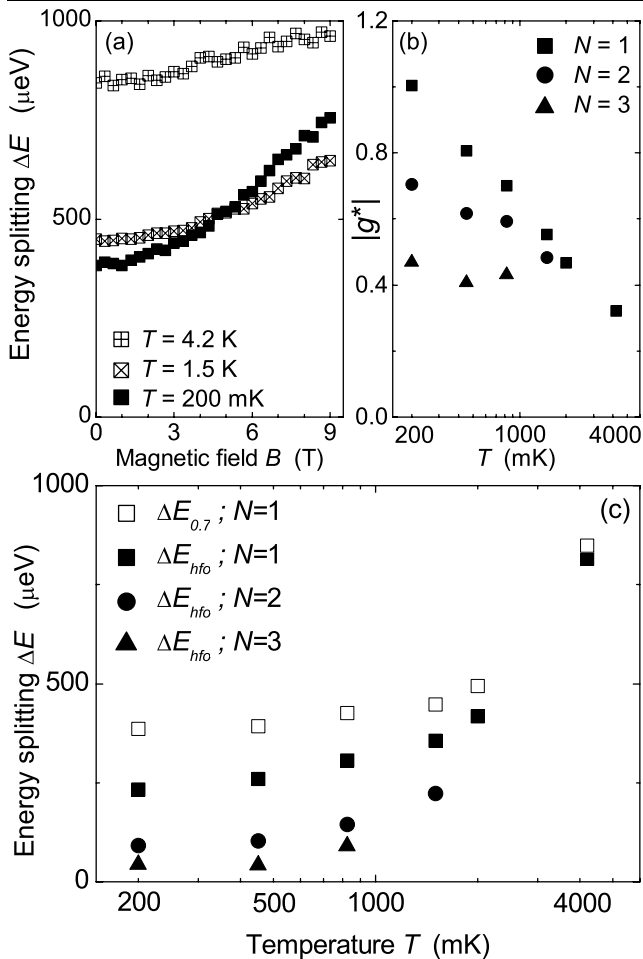
Fig. 6 a Energy splitting for N = 1 as a function of magnetic field for different temperatures T , for a QPC with L = 150 nm and W = 350 nm. b Effective g-factor |g^*| as a function of temperature for the same QPC. The g-factor enhancement is strongest for the N = 1 subband at the lowest temperature. For the N = 2 and N = 3 subband the g-factor is also enhanced at low temperatures. As the temperature is increased the g-factor enhancement is weaker for all subbands. c The 0.7 energy splitting \Delta E_{0.7} and high-field offset \Delta E_{hfo} as a function of temperature. The value for \Delta E_{hfo} is highest for the N = 1 subband and decreases to zero with increasing subband number. As the temperature is increased, the \Delta E_{0.7} value as well as the \Delta E_{hfo} values for N = 1, 2, 3 strongly increase. The correlation between \Delta E_{0.7} and \Delta E_{hfo} remains present upon increasing the temperature
