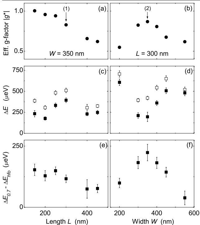
Fig. 4 a, b Effective g-factor |g^*| as a function of QPC length L (with fixed width W = 350 nm), and as a function QPC width W (with fixed length L = 300 nm). The effective g-factor |g^*| is enhanced as compared to the bulk 2DEG value (up to a factor \sim 3 ) and shows a clear dependence on L and W , that is correlated with the dependence of the subband spacing \hbar\omega_{12} in Fig. 3c, d. Data points labeled with (1) and (2) are from two different devices with nominally identical values for L and W (see text for details). c, d The 0.7 energy splitting \Delta E_{0.7} and high-field offset \Delta E_{hfo} for the N = 1 subband as a function of L and W . The values of \Delta E_{0.7} and \Delta E_{hfo} both vary with L and W in an irregular manner, but there is a strong correlation between \Delta E_{0.7} and \Delta E_{hfo} . e, f The difference between \Delta E_{0.7} and \Delta E_{hfo} as a function of L and W . This data again shows a correlation with the dependence of subband spacing \hbar\omega_{12} on L and W . All data points are for the N = 1 subband from results measured at 200 mK (Fig. 3c, d)
