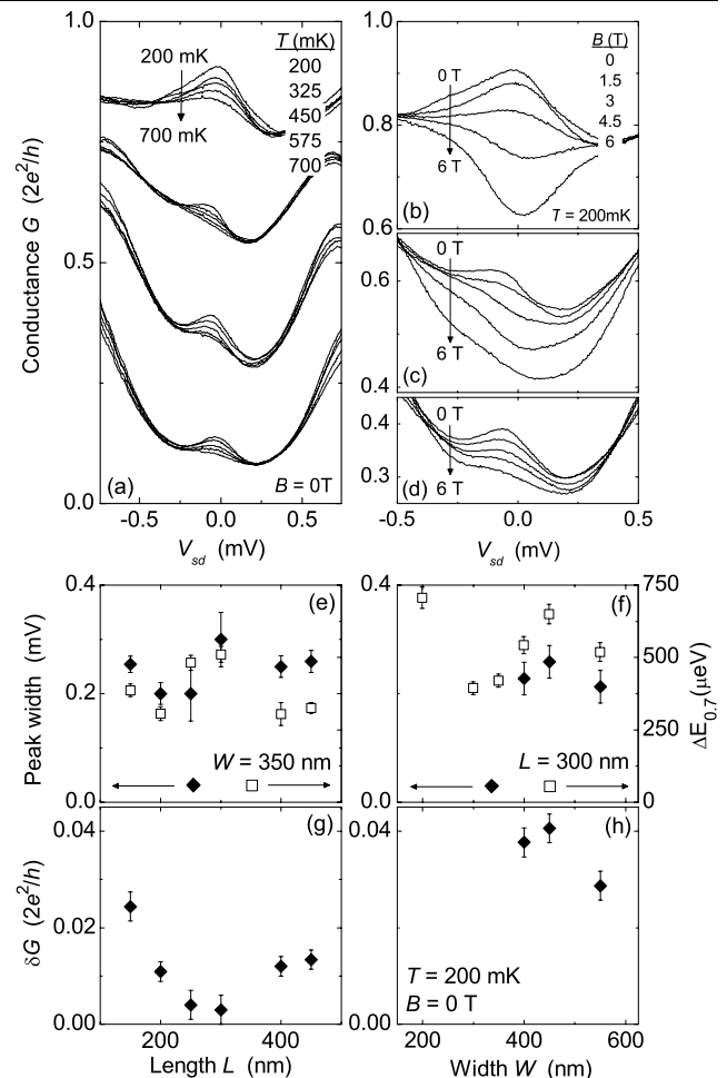
Fig. 7 a Temperature dependence of the zero-bias anomaly (ZBA) for 4 fixed values of the gate voltage. The peak becomes more pronounced as temperature is lowered from 700 to 200 mK. b–d Magnetic field dependence of the ZBA for G \sim 0.8 ( b ), G \sim 0.5 ( c ) and G \sim 0.3(2e^2/h) ( d ). The ZBA should split by upon application of an in-plane magnetic field [13, 32]. The peak in ( b ) does not split but collapses with B because T_K < 2g^*\mu_B B in this regime [13]. The splitting in ( c ) and ( d ) is not very prominent, possibly due to our electron temperature of \sim 200 mK. e, f The width of the ZBA at G \sim 0.3(2e^2/h) (left axis) as a function of QPC length L and width W . The peaks are fitted in zero magnetic field at T = 200 mK. The right axis shows \Delta E_{0.7} (data from Fig. 4g, h). g, h Height of the ZBA also at G \sim 0.3(2e^2/h) versus L and W for the same conditions as in ( e ), ( f )
