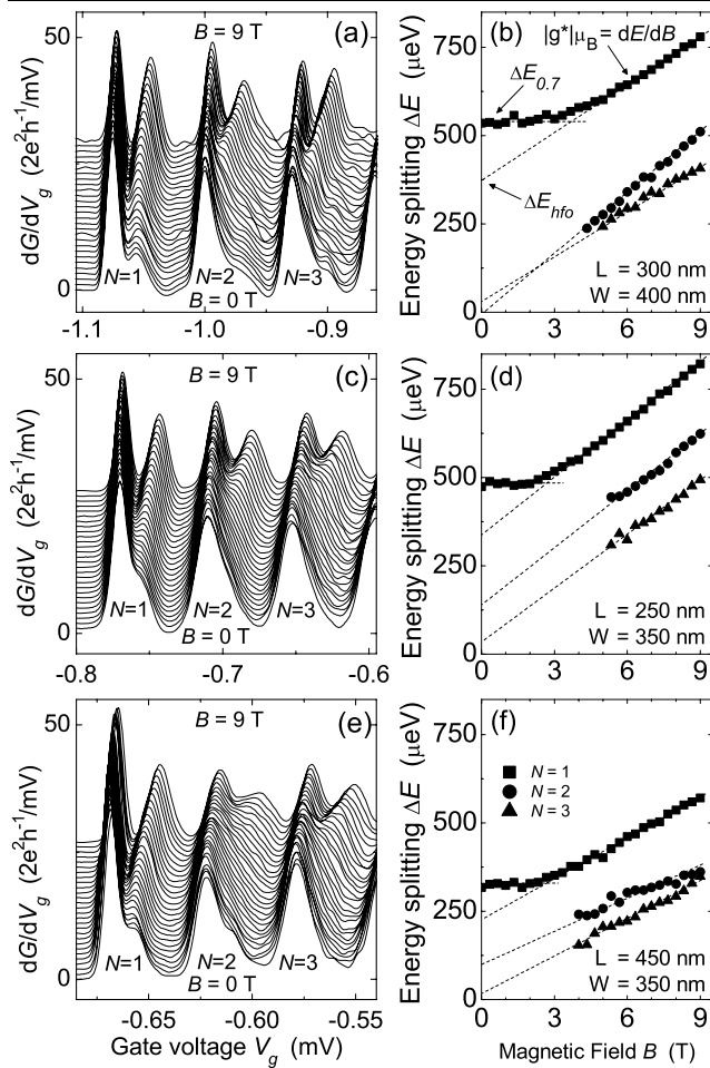
Fig. 2 a Transconductance dG/dV_g traces (offset vertically) obtained from the data in Fig. 1a (from the QPC with L = 300 nm and W = 400 nm). The 0.7 anomaly appears as a splitting of the transconductance peak for the N = 1 subband at B = 0 T. b Energy splittings \Delta E obtained from the transconductance traces in (a), as a function of magnetic field. The traces present \Delta E for the subbands N = 1, 2, 3 , see the legend in (f). These \Delta E traces are characterized (results presented in Fig. 4) with two or three parameters for each subband N = 1, 2, 3 : An effective g-factor |g^*| , the offset from a linear Zeeman effect in high fields, characterized by the high-field offset \Delta E_{hfo} , and for N = 1 at low fields the energy splitting of the 0.7 anomaly, \Delta E_{0.7} . See text for details. c–f Transconductance traces dG/dV_g and energy splittings \Delta E as in (a), (b) obtained for a QPC with L = 250 nm and W = 350 nm in (c), (d) and L = 450 nm and W = 350 nm in (e), (f). All data from measurements at 200 mK
