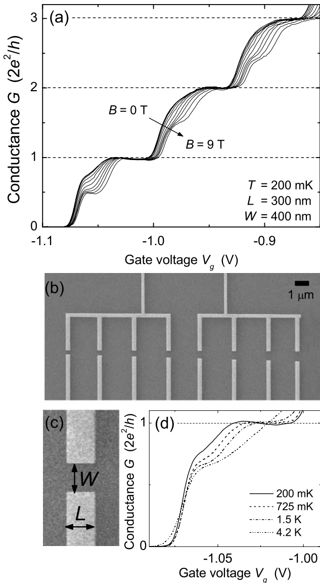
Fig. 1 a The differential conductance G as a function of gate voltage V_g at 200 mK, for a QPC with L = 300 nm and W = 400 nm. The in-plane magnetic field is increased from B = 0 T to B = 9 T. The first three spin-degenerate plateaus at integer multiples of 2e^2/h for B = 0 T split into six spin-resolved plateaus integer multiples of e^2/h for B = 9 T. b Micrograph of a device containing 8 QPCs. From left to right the width W is increased, where W is defined as the spacing between the gate electrodes as shown in (c) . L is the length of the channel. Table 1 contains all values for L and W of the measured devices. d Differential conductance G as a function of gate voltage V_g at zero field for different temperatures. The 0.7 anomaly becomes more pronounced with increasing temperature
