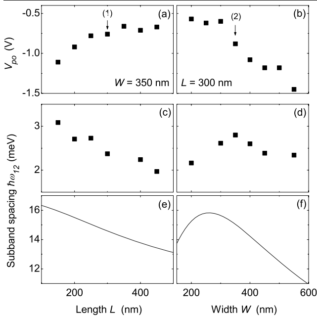
Fig. 3 a, b The pinch-off voltage V_{po} as a function of QPC length L (with fixed width W = 350 nm), and as a function QPC width W (with fixed length L = 300 nm). Data points labeled with (1) and (2) are from two different devices with nominally identical values for L and W (see text for details). c, d The measured subband spacing \hbar\omega_{12} as a function of L and W . e, f Calculated subband spacing \hbar\omega_{12} as a function of L and W , from electrostatic modeling of the QPC potential. The results qualitatively reproduce the trend in the experimental data in (c), (d)
