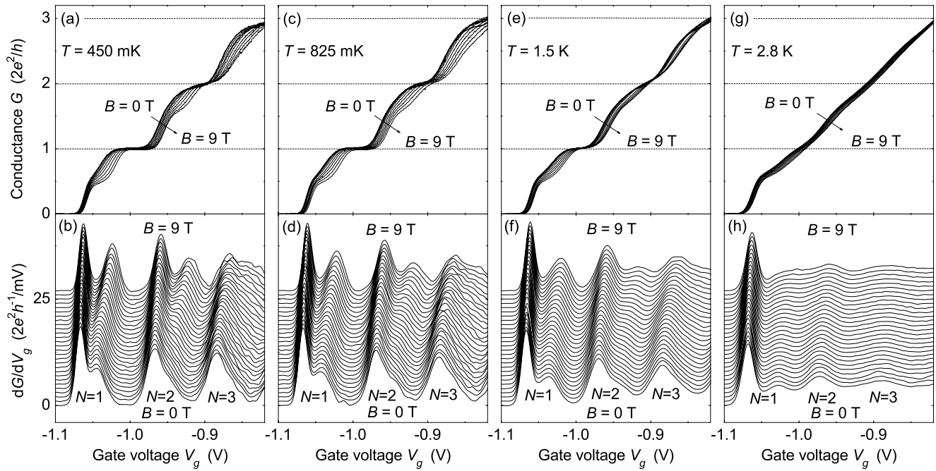
Fig. 5 a Differential conductance G as a function of gate voltage V_g at 450 mK, for a QPC with L = 300 nm and W = 400 nm. The in-plane magnetic field is increased from B = 0 T to B = 9 T. b Transconductance dG/dV_g traces (offset vertically for clarity) obtained by
