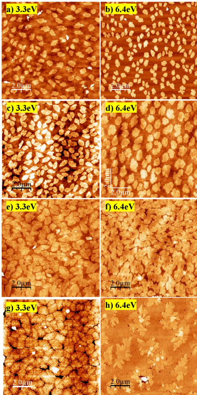
FIG. 1 (color online). AFM micrographs ( 10 \times 10 \mu\text{m}^2 ) of pentacene grown by SuMBD at two kinetic energies: E_k = 3.3 \text{ eV} (first column) and E_k = 6.4 \text{ eV} (second column). The evolution of the deposition has been characterized at different exposure times: (a),(b) at 10 min; (c),(d) at 20 min; (e),(f) at 30 min; (g),(h) at 50 min.
