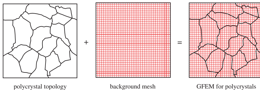
Figure 2. Proposed GFEM approximation of a polycrystal sample.
