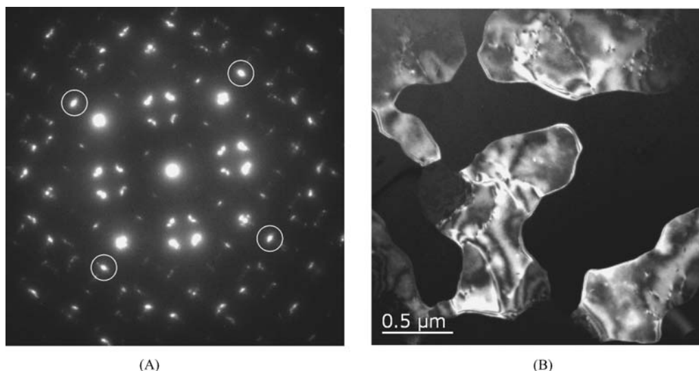
Figure 1 Diffraction pattern (A) and typical two beam dark field image of Al (110) on Si (100) (B). The (02-2) and (2-02) spots from both Al orientations are marked by circles in the diffraction pattern.
