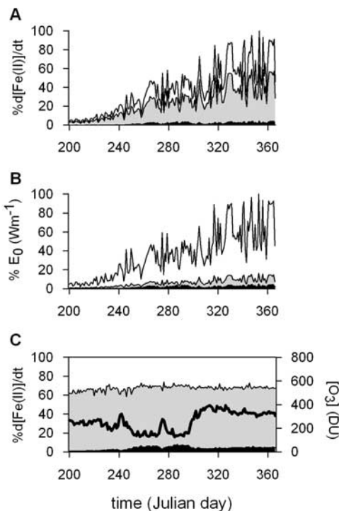
Figure 2. (a) Relative Fe(II) photoproduction rates in the surface ocean as a result of UVB (black), UVA (grey) and VIS (clear) exposure, using solar spectra from 18 July until 31 Dec. 2000 (16:00 GMT). Values were taken as percentage of the highest value for the Fe(II) photoproduction rate. (b) The relative intensities of incident UVB ( \times 10 ) (black), UVA (grey) and VIS (clear) at the sea surface. Values were taken as percentage of the highest measured value for the light intensity. (c) The predicted relative Fe(II) photoproduction rate as a result of UVB (black), UVA (grey) and VIS (clear) and the concentration ozone in Dobson Units (DU) (black line). The Fe(II) photoproduction rates are relative to the Fe(II) photoproduction rate due to total irradiance each day.
