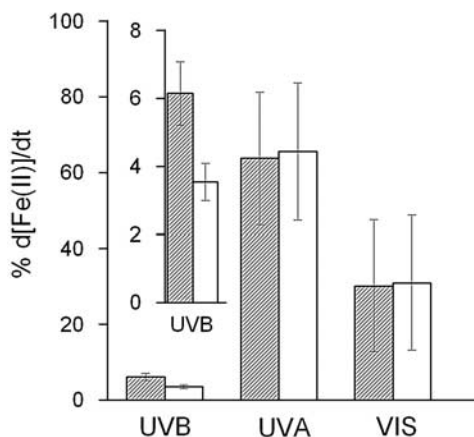
Figure 3. The wavelength band-dependent Fe(II) photoproduction as percentage of the photoproduction due to the total spectrum (280–605 nm) at 23 Sept. 2000 (16:00 GMT) (145.1 DU) and 9 Nov. 2000 (16:00 GMT) (389.9 DU). Incident UVB increased from 0.40% to 0.68% of solar irradiance. Insert: The difference in Fe(II) photoproduction rate due to UVB is significant (3.54% to 6.15%) and due to ozone depletion on 23 Sept. The uncertainty is given as the standard error derived from the weighting function.
