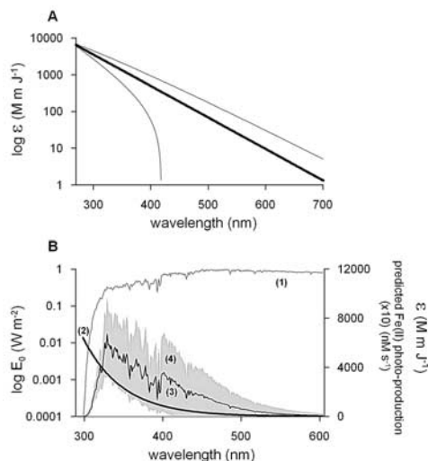
Figure 1. (a) The spectral weighting function ( \log \varepsilon scale) for the photoreduction of Fe in Southern Ocean seawater. The upper and lower lines represent the 95% confidence interval. (b) The solar spectrum (1) ( \log E scale ( \text{W m}^{-2} )), recorded on 22 Nov. 2000 (12:00 GMT) under ozone depleted conditions (370.4 DU), the weighting function (2) ( \varepsilon ( \text{M m J}^{-1} )) and the resulting predicted Fe(II) photoproduction (3) ( (\times 10) \text{nM s}^{-1} ) with its 95% confidence interval (4) (light grey).
