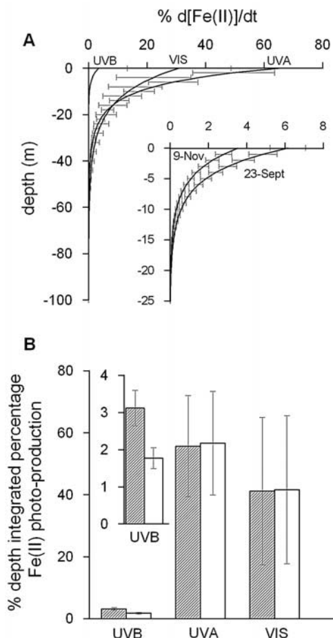
Figure 4. (a) The relative Fe(II) photoproduction rate due to natural UVB, UVA and VIS exposures (9 Nov. 2000, 16:00 GMT) with depth. Insert: The relative Fe(II) photoproduction rate due to UVB at 23 Sept. 2000 (16:00 GMT) (145.1 DU) and at 9 Nov. 2000 (389.9 DU) with depth. Values are expressed as relative to the total irradiance at the surface. (b) The percentage depth integrated Fe(II) photoproduction due to UVB, UVA and VIS for 23 Sept. (hatched) and 9 Nov. (non-hatched). Insert: The significant difference in depth integrated Fe(II) photoproduction due to enhanced UVB during ozone depletion. The uncertainties are given as standard errors derived from both the weighting function and the attenuation coefficients.
