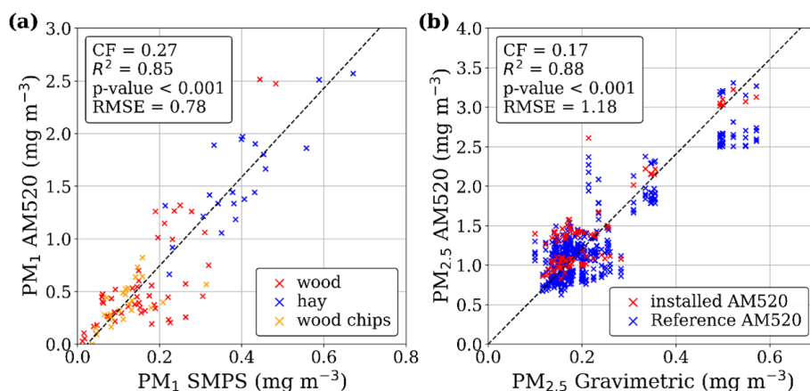
Figure 4. PM 1 concentrations from the AM520 averaged over 160 s plotted against the SMPS-derived PM 1 measurements for 14 fires in different fuel types (a). Fire-averaged PM 2.5 concentrations from five different AM520 modules during 10 experiments burning peat and straw, plotted against the gravimetric measurement from the Tapered Element Oscillating Microbalance (b). The dashed line represents the linear regression line. The VU AM520, shown in red in panel (b), is used for the other analysis in this study.
