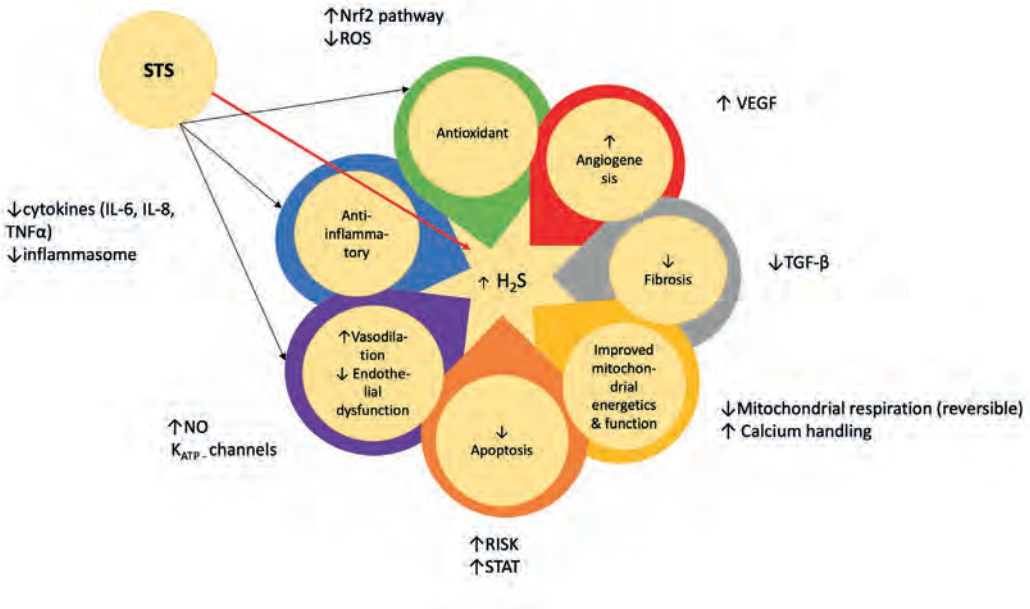
Figure 1 | Schematic overview of cardioprotection by sodium thiosulfate and hydrogen sulfide
