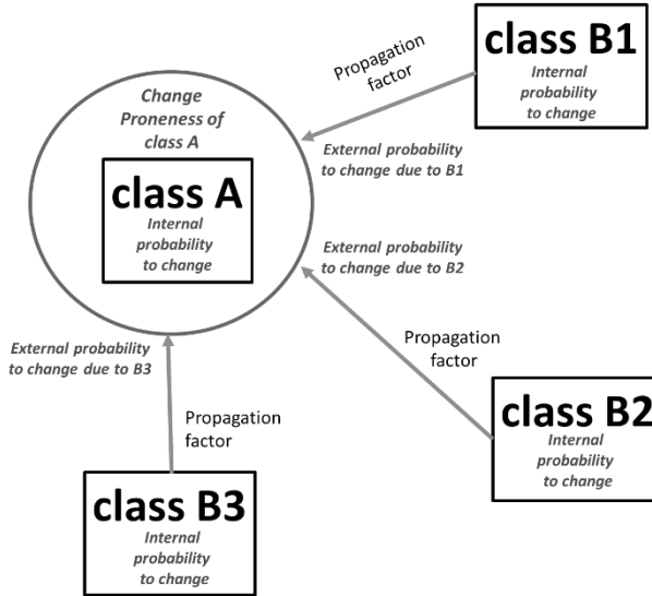
Figure 5.3.a: Rationale of calculation of Change Proneness Metric (CPM)
