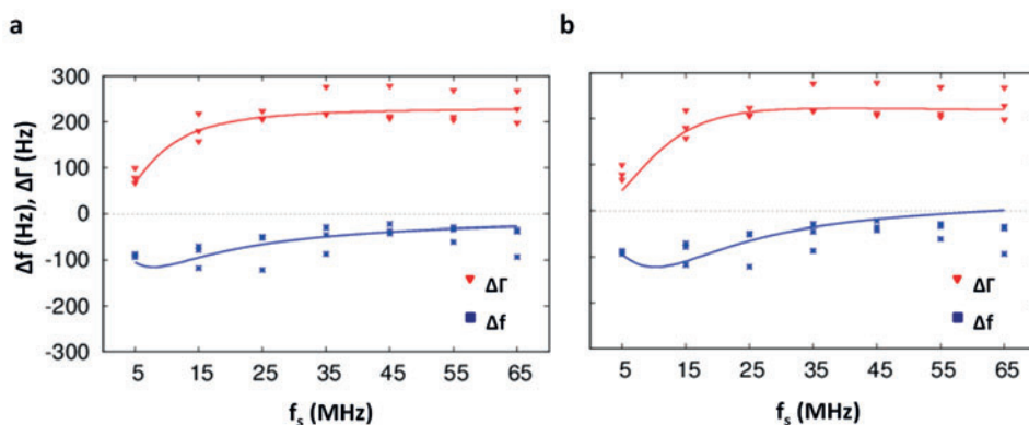
Figure 5. Examples of the QCM-D responses, \Delta f and \Delta \Gamma for adhesion of polystyrene to a hydrophobic SAM crystal surface as a function of the sensor frequency for a) the Kelvin-Voigt model in absence of a polydispersity index and b) the Maxwell model in presence of a polydispersity index.
