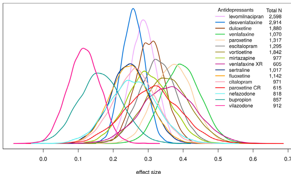
Fig. 2. Posterior effect size differences between drugs.
