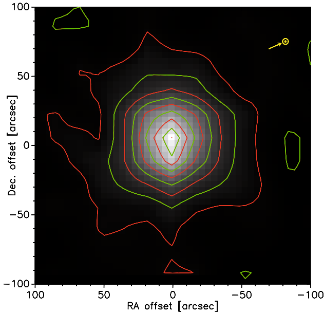
Fig. 4. On-the-fly map of the 557 GHz ortho line obtained by HRS on July 20.95 UT. The contour step is 0.2 \text{ K km s}^{-1} in brightness temperature, from 0 to 1.8 \text{ K km s}^{-1} . The map width is 3 \times 10^5 \text{ km} projected at the comet. The direction towards the Sun is indicated by the arrow in the upper right corner.
