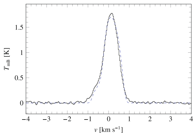
Fig. 1. Spectrum of the 1_{10}-1_{01} ortho-water line at 556.936 GHz in comet C/2008 Q3 (Garradd) obtained by the HRS on July 20.94 UT in FSw mode. The velocity scale is given with respect to the comet rest frame. The dashed line shows a synthetic profile computed with the Monte Carlo model for isotropic outgassing at v_{\text{exp}} = 0.55 km s -1 , T = 15 K, and x_{\text{ne}} = 0.2 .
