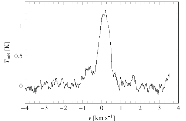
Fig. 2. Average of the HRS frequency-switched observations of the 1_{11}-0_{00} para-water line at 1113.343 GHz in comet C/2008 Q3 (Garradd) obtained on July 22.34 and 27.78 UT.
