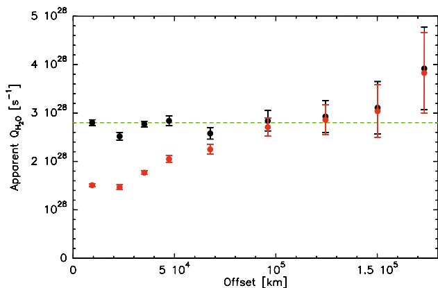
Fig. 6. Apparent water production rates as a function of offset deduced from the 557 GHz map shown in Fig. 4. Isotropic outgassing at v_{\text{exp}} = 0.55 \text{ km s}^{-1} is assumed. Results for x_{n_c} = 0.2 and 1 are shown with black and red symbols, respectively. The dashed horizontal line shows the mean water production rate.
