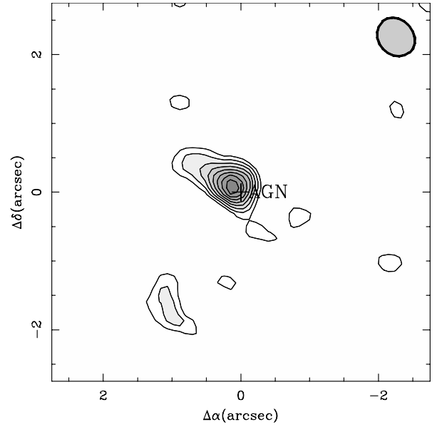
Fig. 2. ^{12}\text{CO}(2-1) intensity map of 3C 236, integrating all emission above 3\sigma levels, from v - v_0 = -685 to +165 km s ^{-1} . The contour levels are 3\sigma , to 6.5\sigma in steps of 0.5\sigma , with \sigma = 0.21 Jy beam ^{-1} km s ^{-1} . (\Delta\alpha, \Delta\delta) -offsets in arcsec are relative to the location of the AGN. The gray ellipse shows the 1 mm beam.
