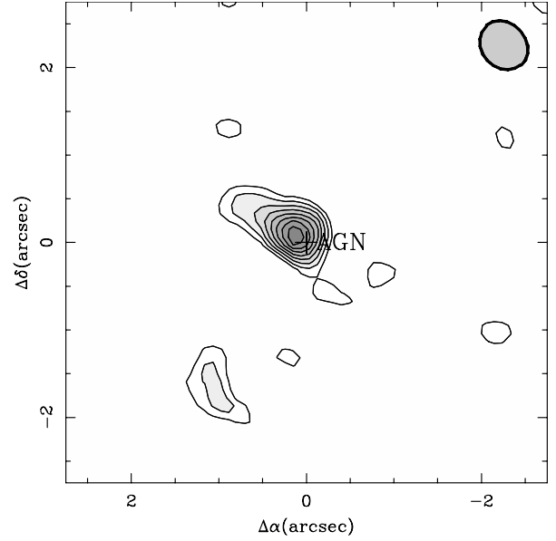
Fig. 2. ^{12}\text{CO}(2-1) intensity map of 3C 236, integrating all emission above 3\sigma levels, from v - v_0 = -685 to +165 km s ^{-1} . The contour levels are 3\sigma , to 6.5\sigma in steps of 0.5\sigma , with \sigma = 0.21 Jy beam ^{-1} km s ^{-1} . (\Delta\alpha, \Delta\delta) -offsets in arcsec are relative to the location of the AGN. The gray ellipse shows the 1 mm beam.
