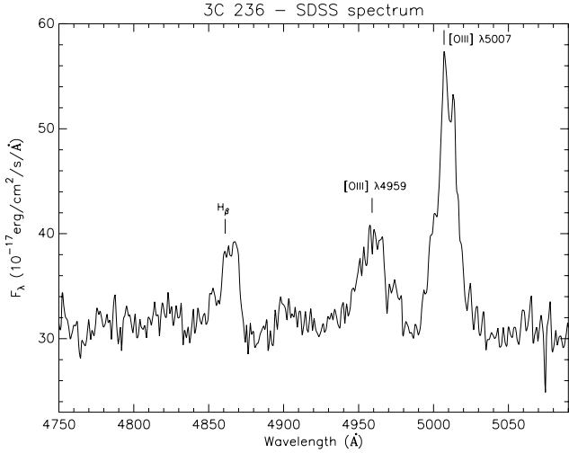
Fig. 7. Optical rest-frame spectrum of 3C 236 from SDSS ( z_{\text{SDSS}} = 0.0991 ). For clarity, we only show the region of the \text{H}\beta and [\text{O III}]\lambda\lambda 4959, 5007 \text{ \AA} emission lines.
