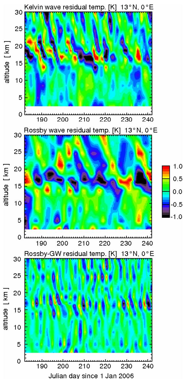
Fig. 8. ECMWF derived residual temperatures from a space-time spectral analysis for (13°N, 0°E) with band pass filters for the different equatorial wave modes applied. The results are shown for Kelvin (top panel), equatorial Rossby (middle panel) and Rossby-gravity waves (bottom panel).
