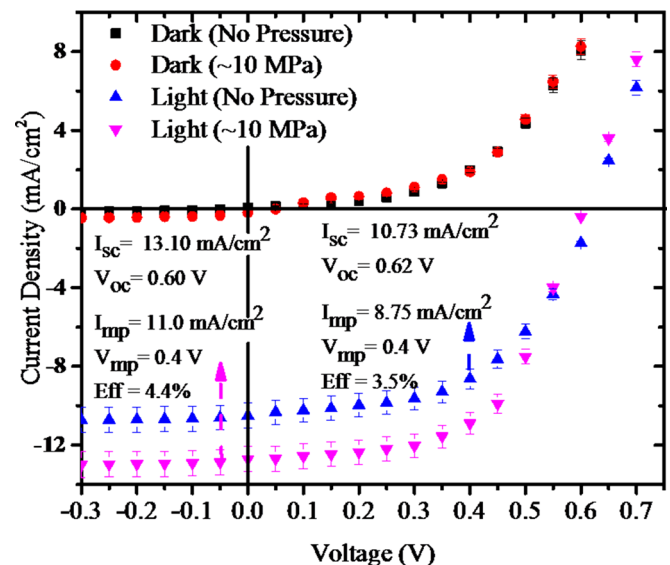
FIG. 9. Power conversion efficiency and current-voltage characteristics of organic photovoltaic devices under pressure application.
