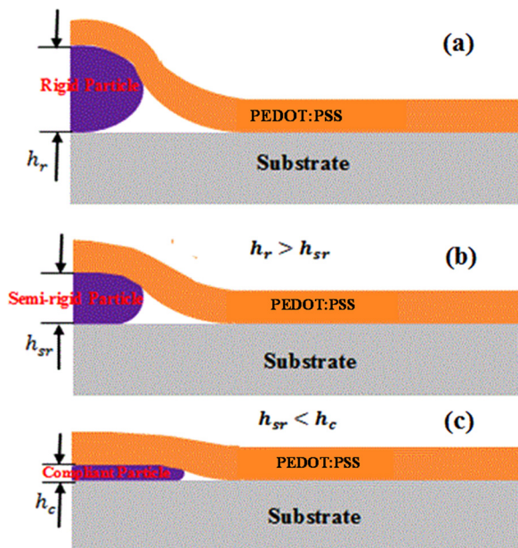
FIG. 8. Schematic diagram of the deformation profiles of trapped particle between the PEDOT:PSS film and the glass substrate with the application of pressure. The height of the particles: rigid, semi-rigid, and compliant are h_r , h_{sr} , and h_c , respectively. 28
