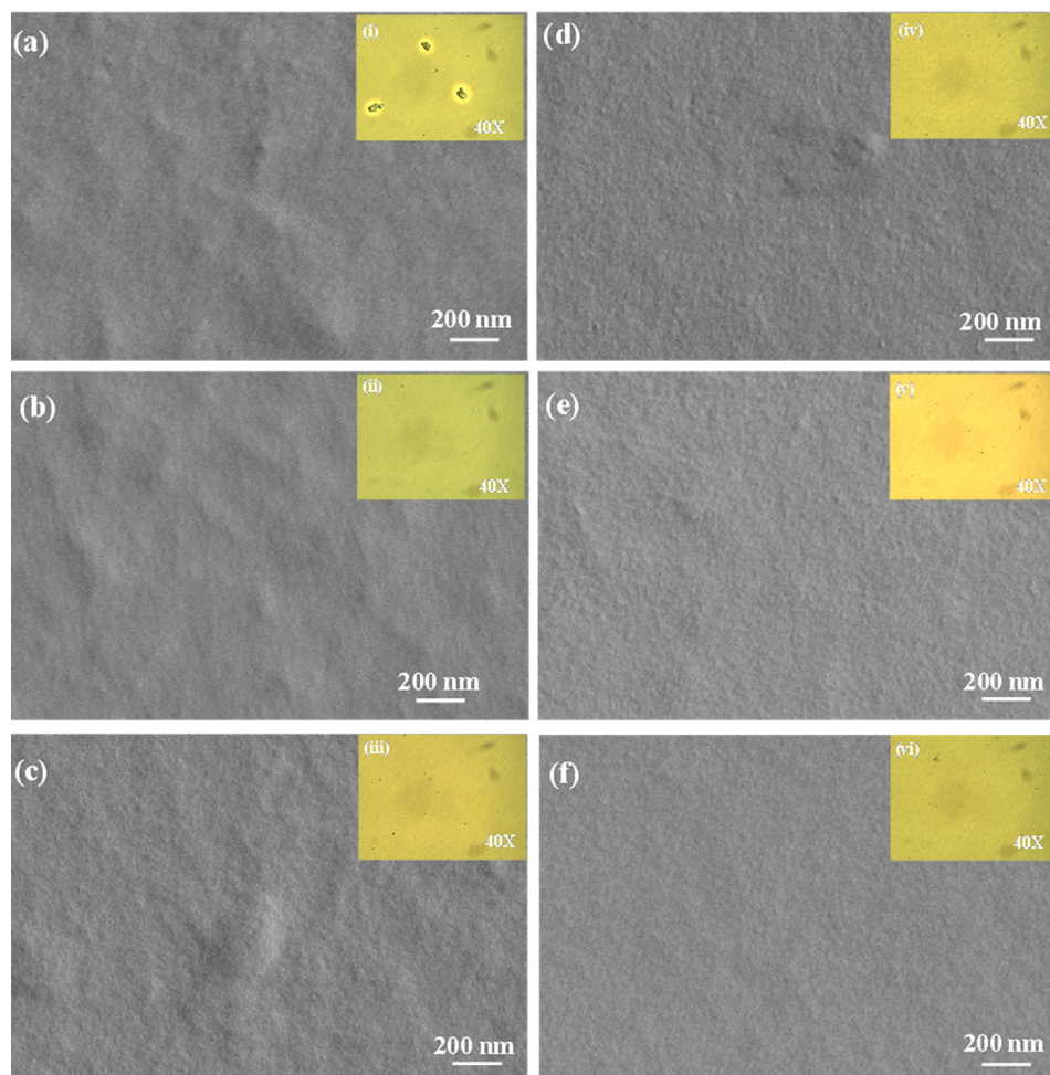
FIG. 2. The surface/interface morphology of the OPV layered structures acquired from the SEM before and after the application of pressure. The images in Figs. 2(a)–2(f) show the rough surfaces increasingly smoothening with pressure to enhance interfacial contacts between the films. Figures: (a) 1 MPa, (b) 3 MPa, (c) 5 MPa, (d) 8 MPa, (e) 10 MPa, and (f) 15 MPa. The insets 2(i)–2(vi) are the optical micrographs of the polymer blends with different applied pressures as above.
