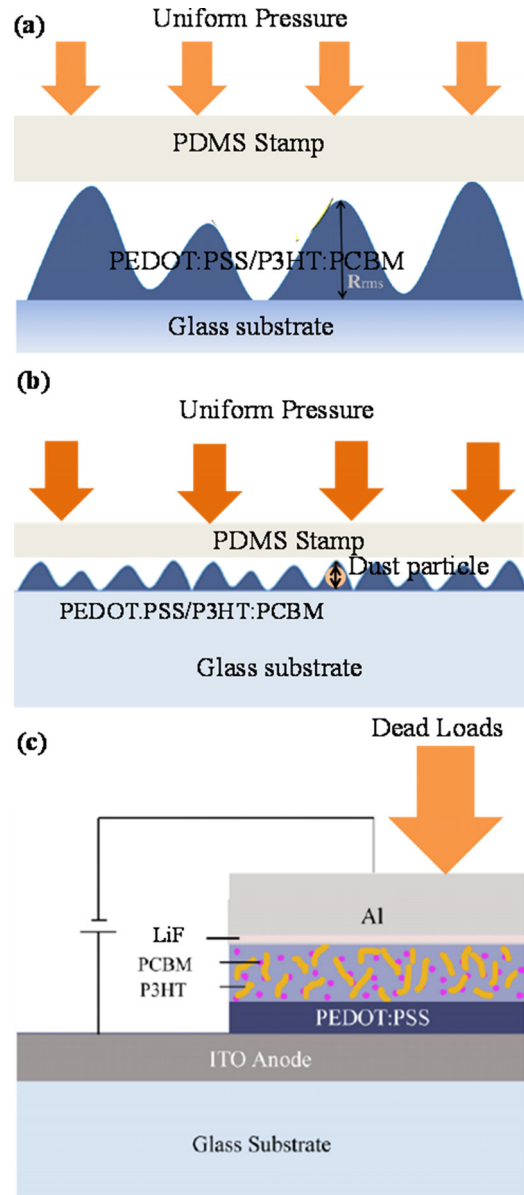
FIG. 1. Bilayered and multilayered nanostructures adopted in the pressure assisted organic photovoltaic cell fabrication: (a) rough surface contacts with blister height, (b) smooth surface contact with trapped particle, and (c) complete device showing multilayers with pressure application.
