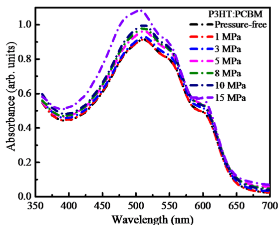
FIG. 4. Shows the ultra-violet-visible (UV-Vis) enhancements in the photo-absorbance of P3HT:PCBM thin films upon the application of pressure. 7,29 The pressure applied include: pressure-less, 1, 3, 5, 8, 10, and 15 MPa.
