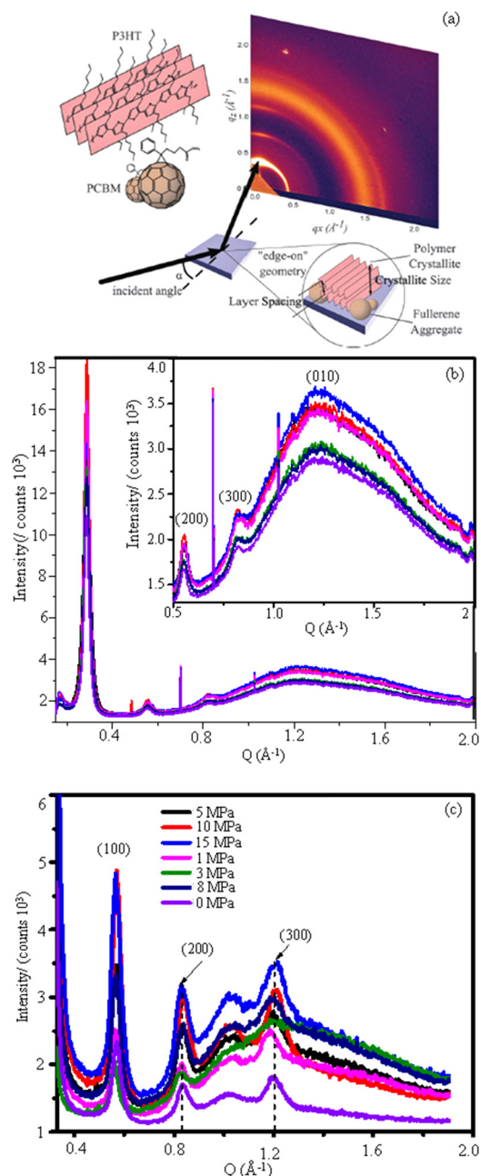
FIG. 3. Polymer crystallinity and chain alignments upon pressure application: (a) GIWAXS representation of the polymer blend-substrate-x-ray interactions, (b) 1D out-of-plane peaks: (100), (200), (300) and in-plane profile showing the (010) dominant peak of P3HT films and (c) the out of plane peak directions [(100), (200), and (300)] indicating the orientation of P3HT crystallites in P3HT:PCBM blends. 21,29,31–35
