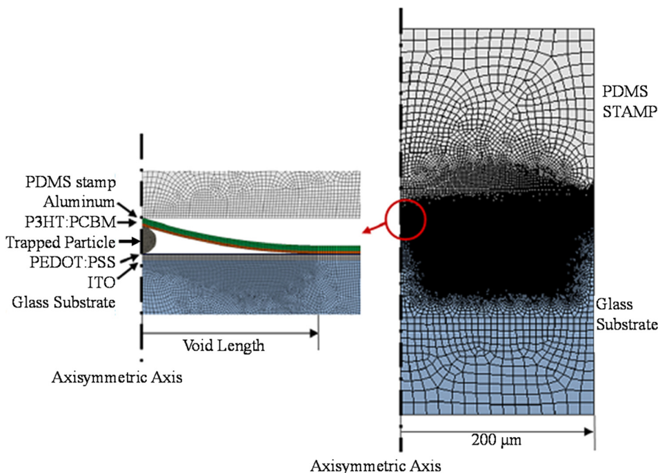
FIG. 6. Finite element model of surface contact during OPV layer deposition with a trapped particle between any two layers. The geometry and mesh show the formation of blisters and the evolution of contact during the pressure application on the PDMS stamp. 5,28
