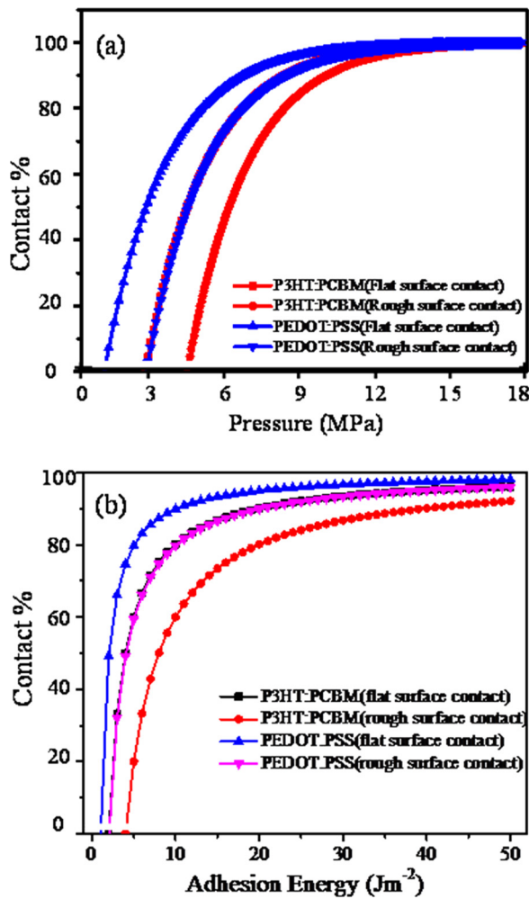
FIG. 5. Analytical modeling of the interfacial surface contacts and their dependence on (a) pressure and (b) adhesion energy between the OPV layers.
