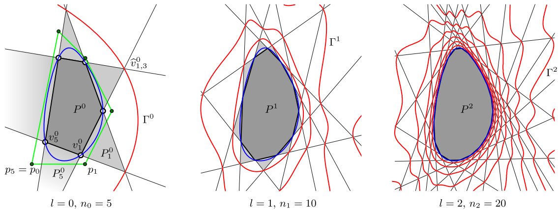
Fig. 3. A sequence of polygons P^l (dark grey) inscribed in a smooth domain \Psi and the associated adjoint curves \Gamma^l (red) for l = 0, 1, 2 . The boundary curve of \Psi (blue) is the periodic uniform cubic B-spline curve defined by the green control polygon. The adjoint curves touch \hat{P}^l (light grey) at the exterior intersection points \hat{v}_{-1,i+1}^l , but do not intersect \hat{P}^l . (For interpretation of the references to colour in this figure legend, the reader is referred to the web version of this article.)
