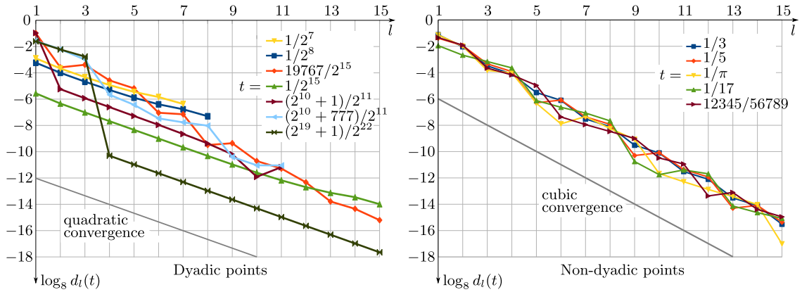
Fig. 7. Behaviour of the interpolated values at dyadic (left) and non-dyadic (right) boundary points for the example in Figs. 3 and 4. Since d_l(t) = 0 for l > k at the dyadic points t = i/2^k , some of the sequences in the left plot are truncated accordingly.
