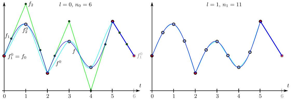
Fig. 6. Approximation of the closed B-spline function f (blue) defined by the green control values over the boundary of \Psi (see Fig. 5) with three “corners” (red bullets) and a linear segment (thick blue) by the restrictions f^l (cyan) of the discrete Wachspress interpolants to \partial\Psi for l=0, 1 . (For interpretation of the references to colour in this figure legend, the reader is referred to the web version of this article.)
