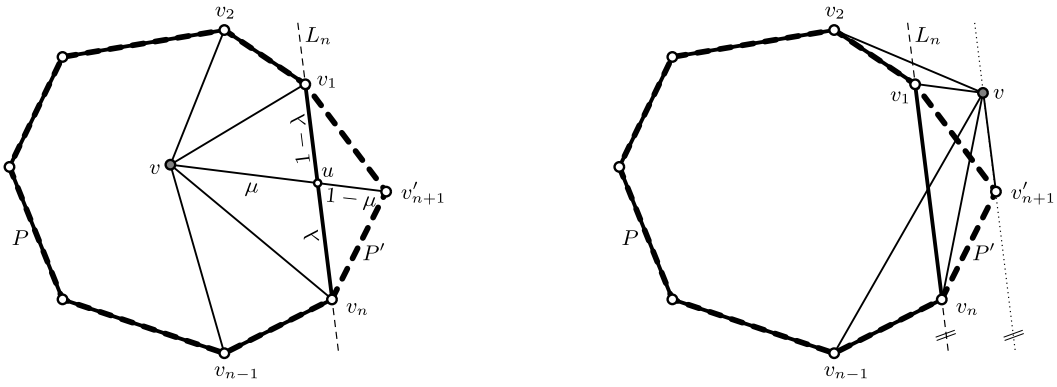
Fig. 2. Notation used in the proof of Lemma 2. The polygon P is marked by thick solid lines, and its refinement P' by thick dashed lines.
