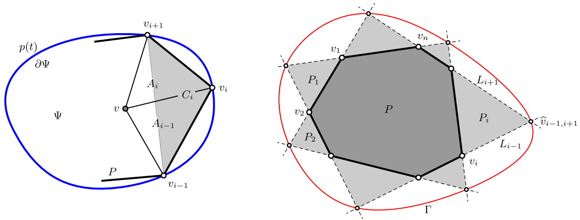
Fig. 1. Left: Notation used in the definition of Wachspress coordinates and the Wachspress kernel, where C_i is the area of the shaded triangle. Right: Notation used to prove our main result.
