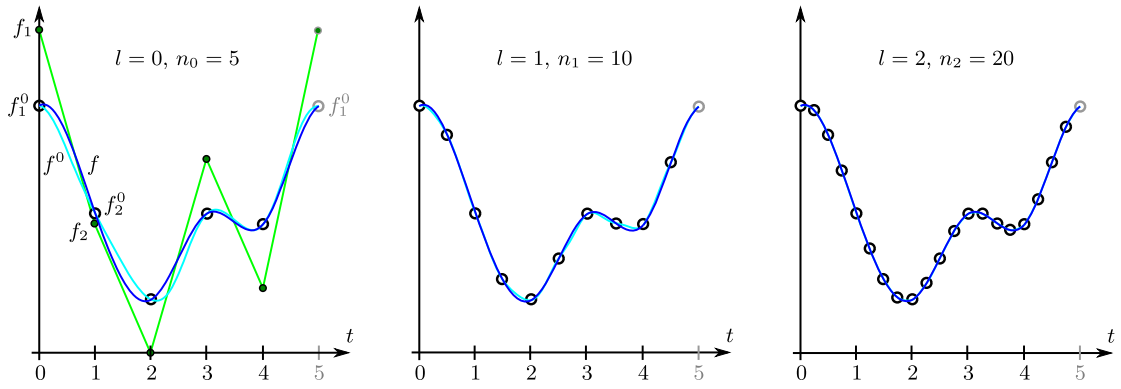
Fig. 4. Approximation of the periodic uniform B-spline function f (blue) defined by the green control values over the boundary of \Psi (see Fig. 3) by the restrictions f^l (cyan) of the discrete Wachspress interpolants to \partial\Psi for l=0, 1, 2 . (For interpretation of the references to colour in this figure legend, the reader is referred to the web version of this article.)
