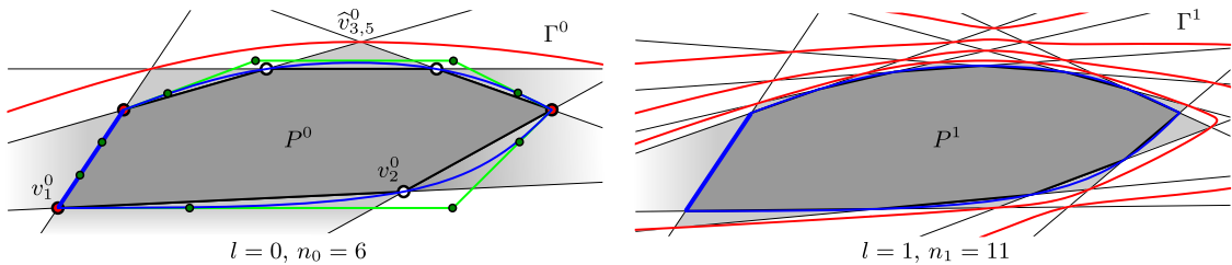
Fig. 5. Admissible polygons P^l (dark grey) inscribed in a weakly convex domain \Psi and the associated adjoint curves \Gamma^l (red) for l=0, 1 . The boundary curve of \Psi (blue) is a closed cubic B-spline curve defined by the green control polygon with three corners (red bullets) and a straight segment (thick blue). The adjoint curves touch P^l (light grey) at the exterior intersection points \hat{v}_{i-1,i+1}^l , but do not intersect P^l . (For interpretation of the references to colour in this figure legend, the reader is referred to the web version of this article.)
