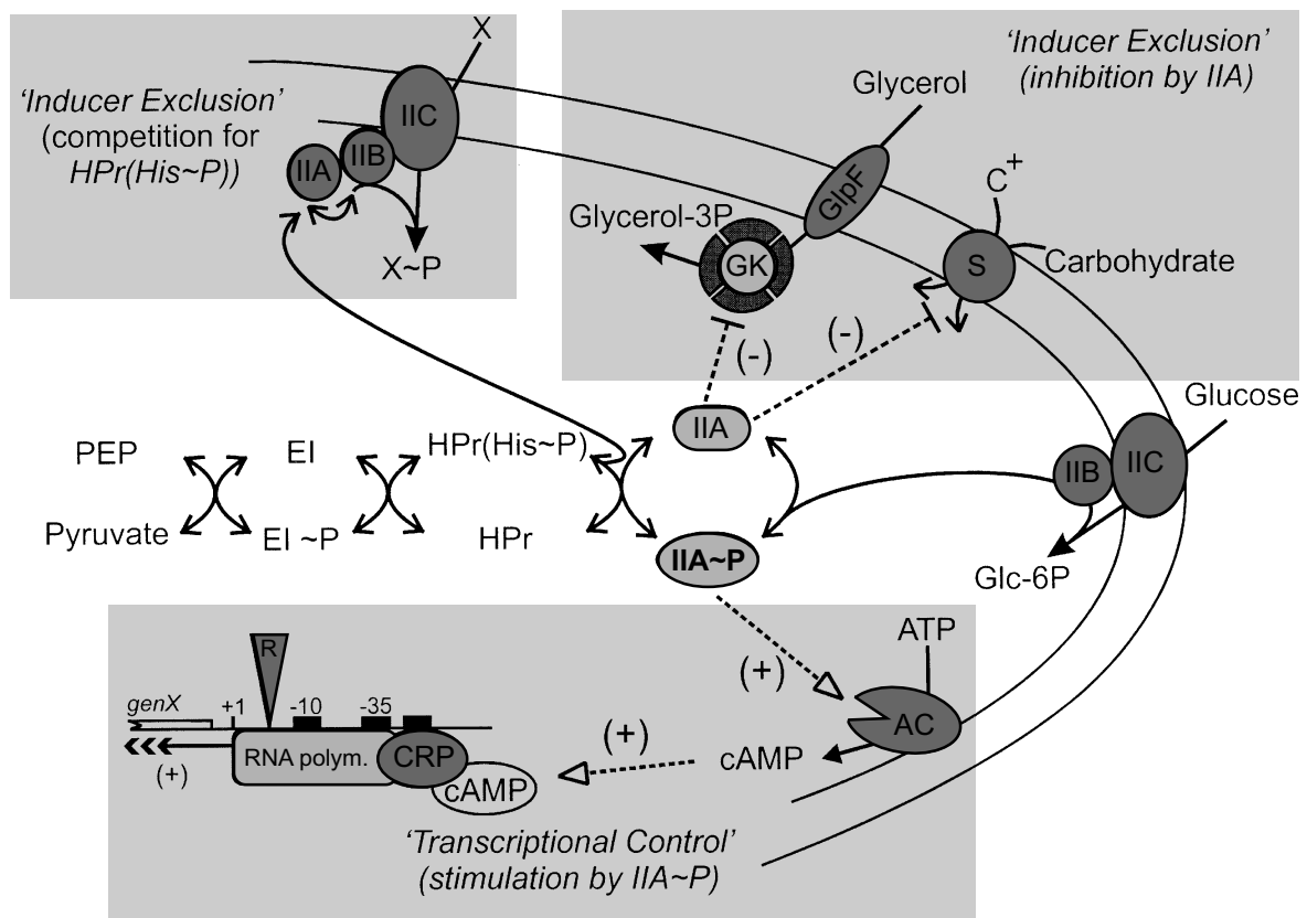
Figure 1. Schematic representation of the phosphoenolpyruvate:glucose phosphotransferase system of Gram-negative enteric bacteria. The central role of \text{IIA}^{\text{Glc}}\text{-P} in controlling transcription and inducer exclusion is illustrated. EI, Enzyme I; Glc-6P, glucose-6P; CRP, cAMP receptor protein; RNA polym., RNA polymerase; R, repressor; \text{C}^+ , cation; S, secondary transport protein; GK, glycerol kinase; and GlpF, glycerol facilitator.
