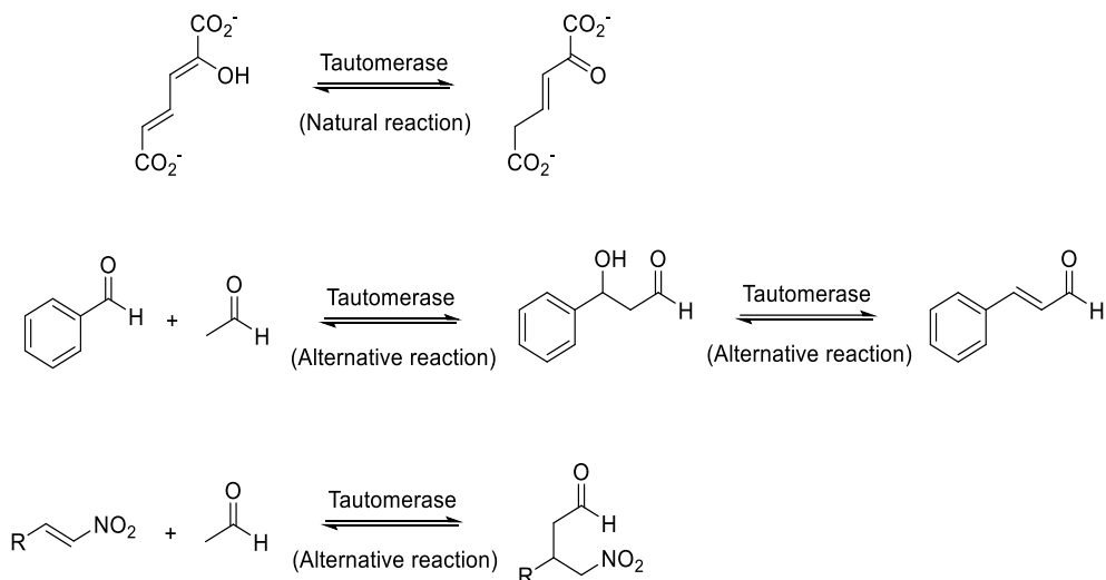
Scheme 1.1: An enol-keto tautomerase also catalyzes C-C bond-forming aldol condensation and Michael-type addition reactions.
