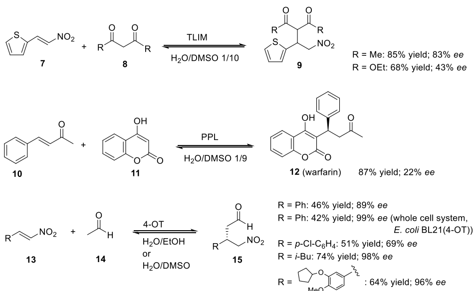
Scheme 1.2: Enzyme promiscuity for asymmetric carbon-carbon bond-forming Michael(-type) additions.
