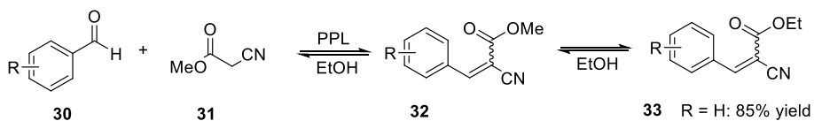
Scheme 1.5: Enzyme promiscuity for Knoevenagel condensations.
