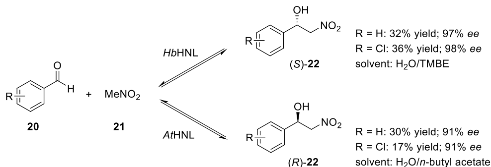
Scheme 1.4: Enzyme promiscuity for asymmetric Henry reactions.
