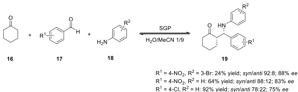
Scheme 1.3: Enzyme promiscuity for asymmetric Mannich reactions.
