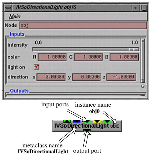
Figure 4: Metaclass icon with ports (left) and its automatically constructed GUI (right)
