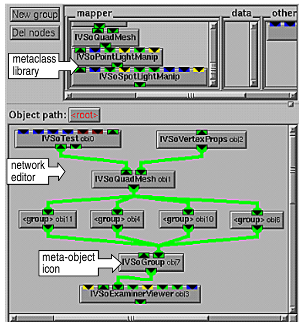
Figure 3: The dataflow network is build in the visual editor by instantiating the loaded metaclasses
