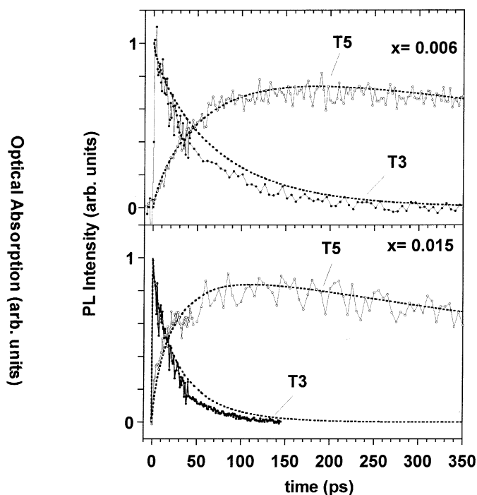
Fig. 3. PL transients of T3 and T5 for x=0.006 and x=0.015 . Numerical simulations (dotted lines) following the model described in the text from Eq. (6). The PL data for times longer than 40 ps have been recorded using a streak camera.
