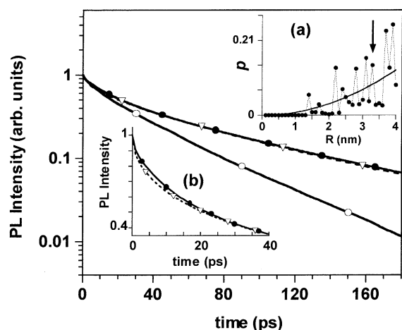
Fig. 5. Numerical simulations of T3 PL transients for x=0.015 from Eq. (6) by including (open circles) and neglecting (solid circles) the D–D homotransfer; and the analytical solution (dotted line, triangles) from Eq. (7) for parallel dipole orientations. In the inset (a), the probability p of finding an acceptor at a distance R from the excited donor is shown for x=0.015 , both for the continuous (solid line) and the discrete distributions (points). The arrow indicates the Foerster radius position. In the inset (b) an enlargement of the heterotransfer short time decays is shown from Eqs. (6) and (7).
