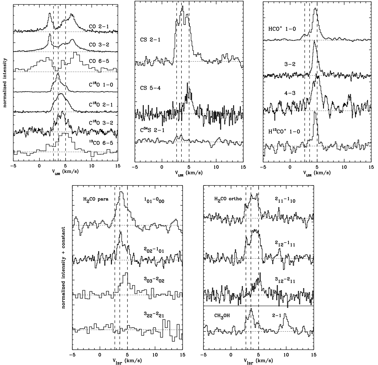
FIG. 3.— Emission lines of CO, CS, HCO + , H 2 CO, and CH 3 OH toward Elias 29. Vertical dashed lines indicate different dynamic components at V_{\text{LSR}}=2.7, 3.8 and 5.0 \text{ km s}^{-1} . The spectra have been arbitrarily scaled and shifted along the intensity axis. See Table 3 for line intensities.
