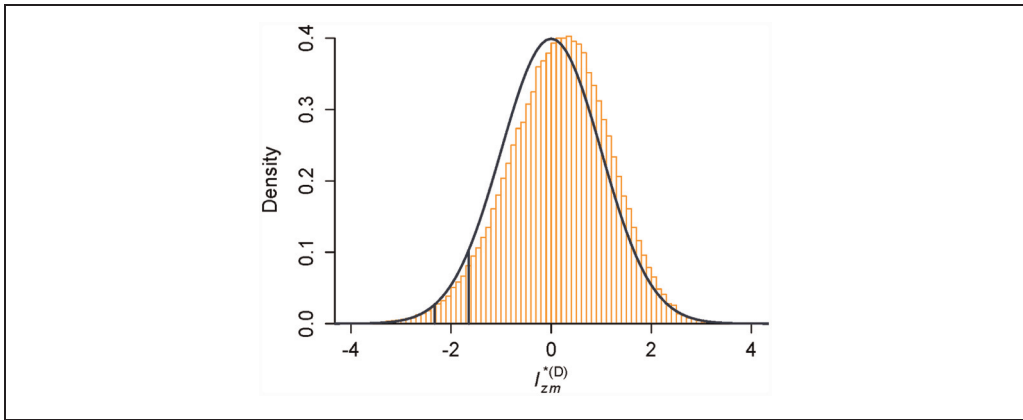
Figure 1. Histogram of the 1,000 \times 100 = 100,000 computed I_{zm}^{*(D)} values (bars) and the standard normal distribution (curve).
