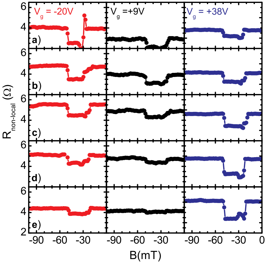
Figure 8.3: The drift effect in a graphene spin valve. The gate voltage V_g varies from left to right and it is indicated for each column. The DC electric current varies from top to down as: (a) I_{DC} = -40 \mu\text{A} , (b) -20 \mu\text{A} , (c) 0 \mu\text{A} , (d) +20 \mu\text{A} , (e) +40 \mu\text{A} . For clarity only the negative side of the spin valve measurements are plotted.
