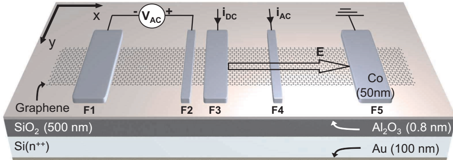
Figure 8.1: Schematic drawing of the spin drift experiment. The Co contact widths are 350 nm (for F1), 90 nm (F2), 250 nm (F3), 90 nm (F4), 350 nm (F5) and the distances between them are (from left to right) 2 \mu\text{m} , 0.6 \mu\text{m} , 1.3 \mu\text{m} and 2 \mu\text{m} . The 0.9 \times 7 \mu\text{m}^2 sized graphene flake is covered by an aluminum oxide layer. A (gate) voltage, applied between the Au contacted Si( n^{++} ) substrate and the grounded electrode F5, allows for the control of the charge density in graphene. The layer thicknesses are given in the brackets.
