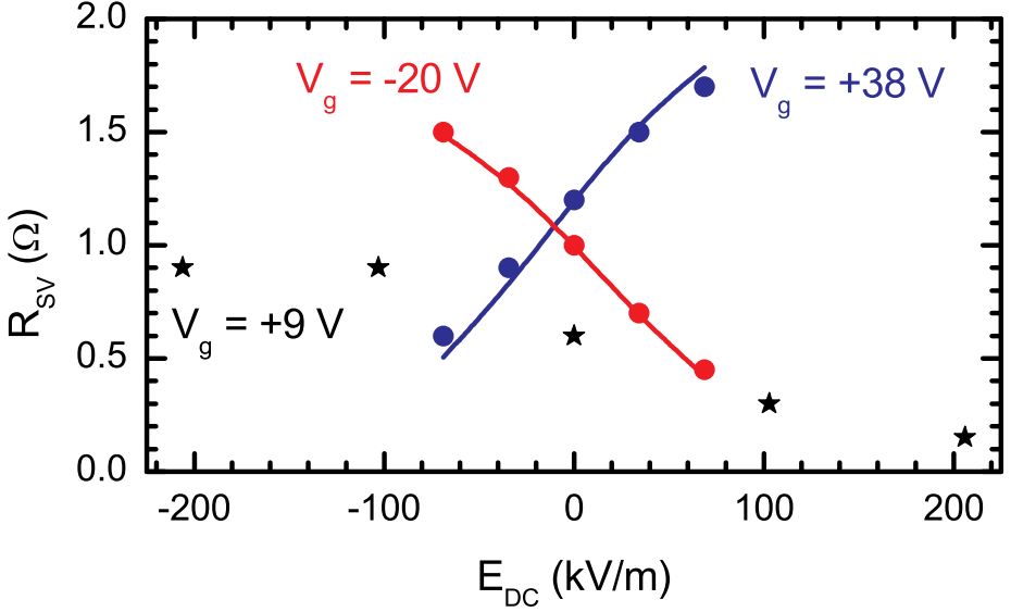
Figure 8.4: Spin valve signal for high carrier densities (circles), and near the Dirac neutrality point (stars). The lines represent a calculation (with no free parameters) of the drift effect based on the drift-diffusion equation.
