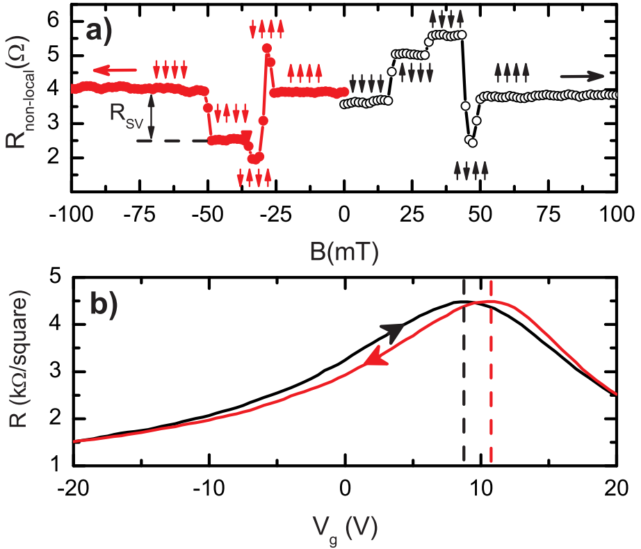
Figure 8.2: a) Non-local spin valve measurement of the device presented in Fig. 8.1. The small arrows represent the magnetic orientation of electrodes F1, F2, F4 and F5. The asymmetric spin valve behavior is due to the switching order of F4 and F5 which depends on external field sweep direction (indicated by the large horizontal arrows). R_{SV} represents the spin signal; see text for details. b) 4-point measurement of the graphene resistivity between contacts F3 and F4 versus the gate voltage.
