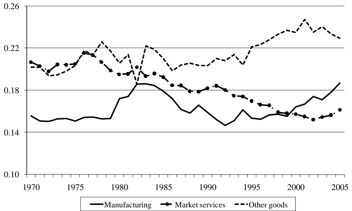
Figure 1, Standard deviation of productivity levels, 1970-2005
