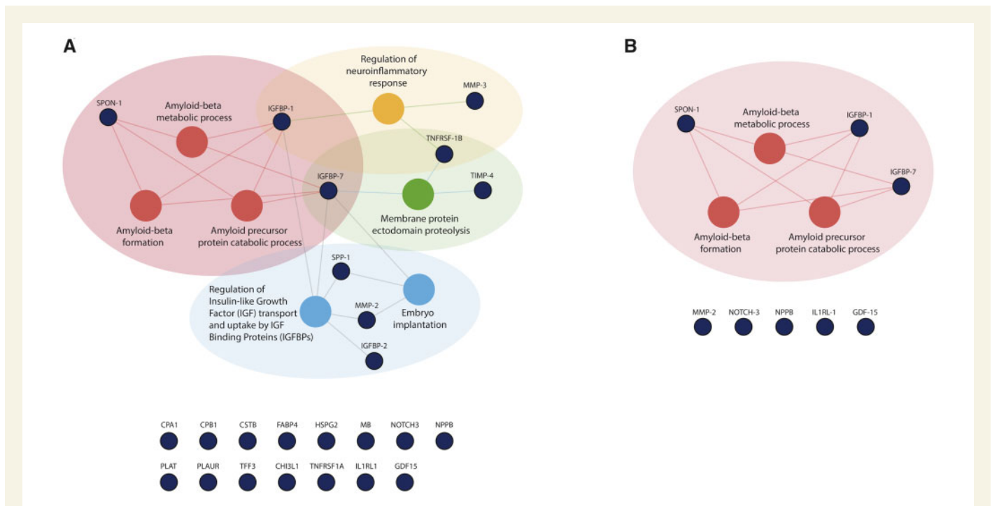
Figure 3 Results of pathway overrepresentation analyses of patients with atrial fibrillation vs. sinus rhythm in the index cohort (A, n = 1620 ) and the validation cohort (B, n = 1219 ) of BIostat-CHF. The nodes in blue represent the 24 biomarkers that were significantly up-regulated in patients with atrial fibrillation when compared with those in sinus rhythm in the index cohort (A), and eight biomarkers that were significantly up-regulated in these patients in the validation cohort (B). The nodes in red reveal the overrepresented pathways of these biomarkers. Based on current knowledge, the blue nodes below the figures are biomarkers that were not found to be overrepresented in a specific biological pathway. CHI3L1, chitinase 3 like 1; CPA1, carboxypeptidase A1; CPB1, carboxypeptidase B1; CSTB, cystatin B; FABP4, fatty acid-binding protein 4, adipocyte; GDF-15, growth differentiation factor 15; HSPG2, heparan sulphate proteoglycan 2; IGFBP-1, insulin like growth factor binding protein 1; IGFBP-2, insulin-like growth factor-binding protein 2; IGFBP-7, insulin like growth factor binding protein 7; IL1RL1-1, interleukin 1 receptor like 1; MB, myoglobin; MMP-2, matrix metalloproteinase 2; MMP-3, matrix metalloproteinase 3; NOTCH3, neurogenic locus notch homolog protein 3; NPPB, natriuretic peptide B; PLAT, plasminogen activator, tissue type; PLAUR, plasminogen activator, urokinase receptor; SPON-1, spondin-1; SPP-1, secreted phosphoprotein 1; TFF3, trefoil factor 3; TIMP-4, metalloproteinase inhibitor 4; TNFRSF1A, TNF receptor superfamily member 1A; TNFRSF1B, TNF receptor superfamily member 1B.
