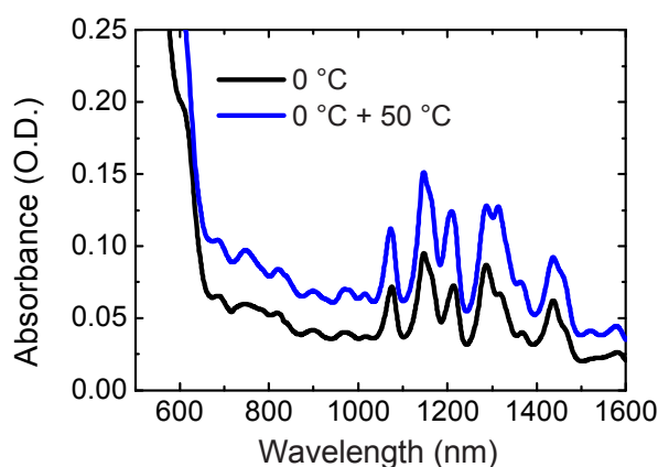
Figure 3.7 Absorption spectra after centrifugation of P3DDT-SWNTs obtained from polymer solutions without-aggregation sonicated at 0\text{ }^{\circ}\text{C} with and without thermal treatment at 50\text{ }^{\circ}\text{C} before centrifugation.
