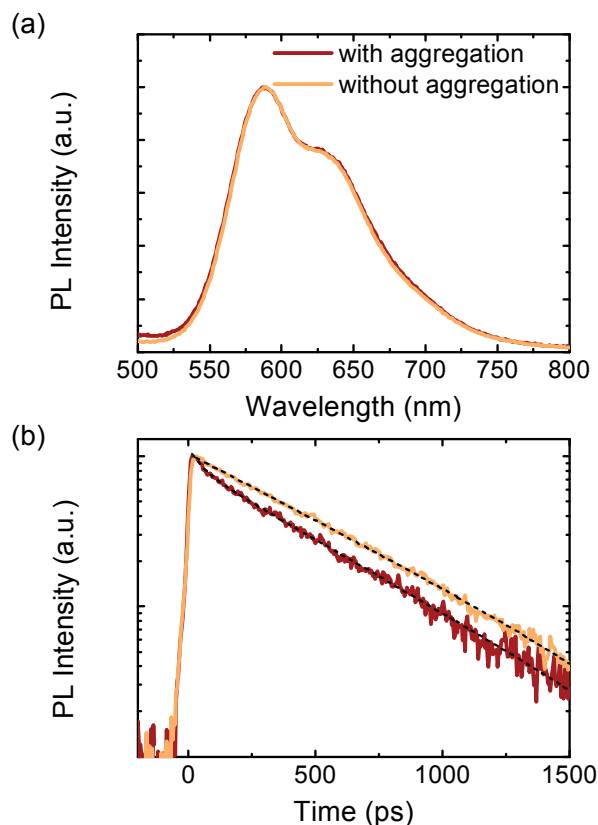
Figure 3.3 (a) Photoluminescence spectra (polymer component) of P3DDT-wrapped SWNT dispersions after complete free polymer removal, obtained from polymer solutions with- and without-aggregation. (b) Time resolved photoluminescence of the samples as in (a) measured at 580 nm. The dashed black lines are the fittings of the experimental data.
