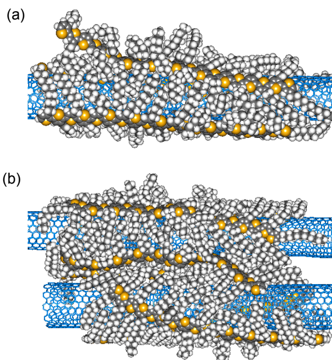
Figure 3.5 Assembly of P3DDT polymers on nanotubes in toluene solutions (toluene not shown for clarity). Carbon nanotubes are represented by the blue structures, and the polymers by overlapping spheres: yellow=S, gray=C, white=H. (a) (12,7) nanotube wrapped by 3 polymer chains; (b) a dyad of (12,10) and (10,9) SWNTs wrapped by 7 polymer chains.
