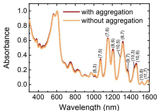
Figure 3.2 Normalized absorption spectra of polymer-wrapped SWNT dispersions after complete free polymer removal prepared with P3DDT with- and without-aggregation. The assignment of the chiralities follow previously reported literature data. [5]
