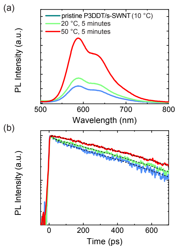
Figure 3.4 Comparison of the polymer photoluminescence spectra (a) and decays (b) in s -SWNTs wrapped with P3DDT after complete free polymer removal, obtained from solution with-aggregation at 10 °C (blue curve); after sample treatment at 20 °C for 5 minutes (green curves); after thermal treatment at 50 °C for 5 minutes (red curve). The black dashed lines are the fittings to the experimental curves.
