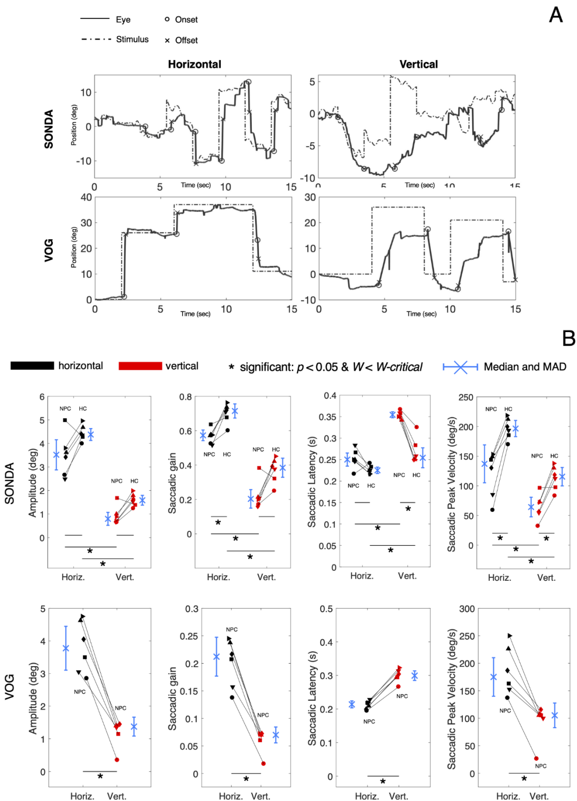
Fig. 1. Conventional saccadic parameters (amplitude, gain, latency, and peak velocity) in SONDA and VOG. A. Time-series of gaze data obtained with SONDA (upper panel) and VOG (lower panel). The stimuli had comparable spatial ranges, leading to saccades with amplitudes prevalently between 0 deg and 20 deg. Both methods showed a robust identification of visually evoked saccades. B. Comparisons of conventional saccadic parameters between NP-C patients and age-matched controls, and between horizontal and vertical saccades, measured with SONDA and VOG. On each scatterplot, the blue X mark is the median, the error bars are the Mean Absolute Deviations. The black horizontal lines indicate the pair-wise comparisons used for statistical testing. Each age-matched patient-control pair is indicated by connected dots with matching symbols. (For interpretation of the references to colour in this figure legend, the reader is referred to the web version of this article.)
