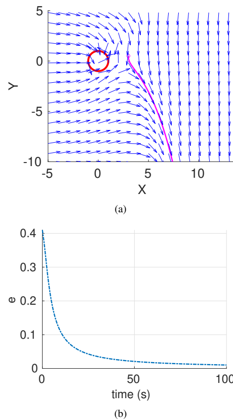
Fig. 2. The desired set \mathcal{A} is a unit circle illustrated by a red curve in (a), and in this subfigure, the arrows represent the normalized vector field computed by (2). Although the level value e = \phi = (x^2 + y^2 - 1)\exp(-x) converges to 0 in (b), the trajectory given by the magenta curve in (a) escapes to infinity.
