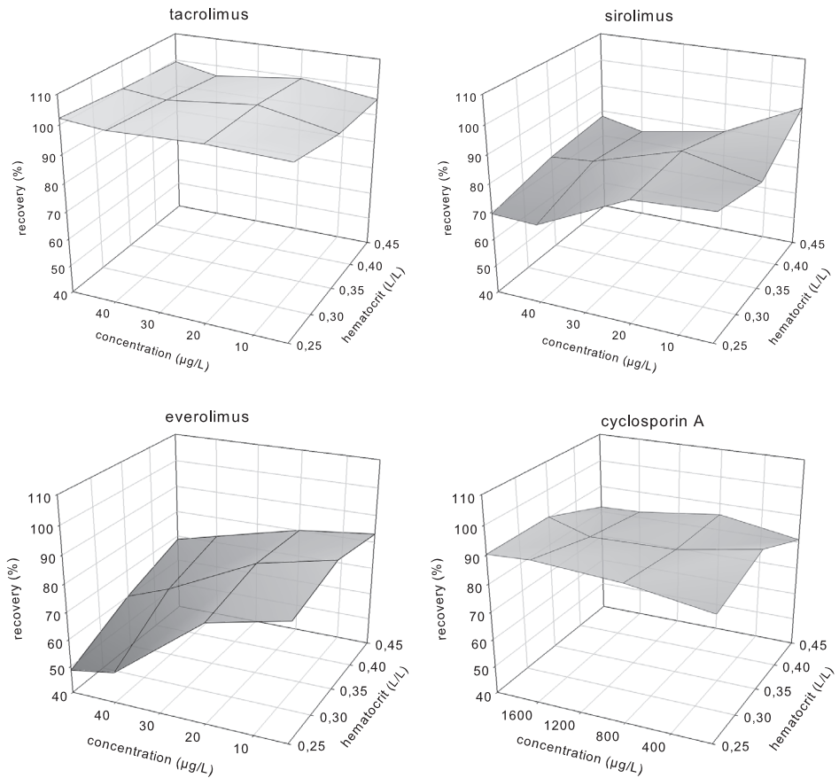
Figure 2 Recoveries of tacrolimus, sirolimus, everolimus and cyclosporin A influenced by concentration and HT, without the chromatographic effect of the paper.
