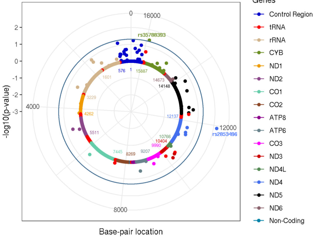
Figure 1. Solar Manhattan plot of the association between mitochondrial DNA variants and primary open-angle glaucoma. Each dot represents a variant association, coded by gene. The positions of the variants are on a circular x-axis. The -\log_{10}(p) -values are on a radial y-axis and the blue circle indicates p -values = 0.05.
