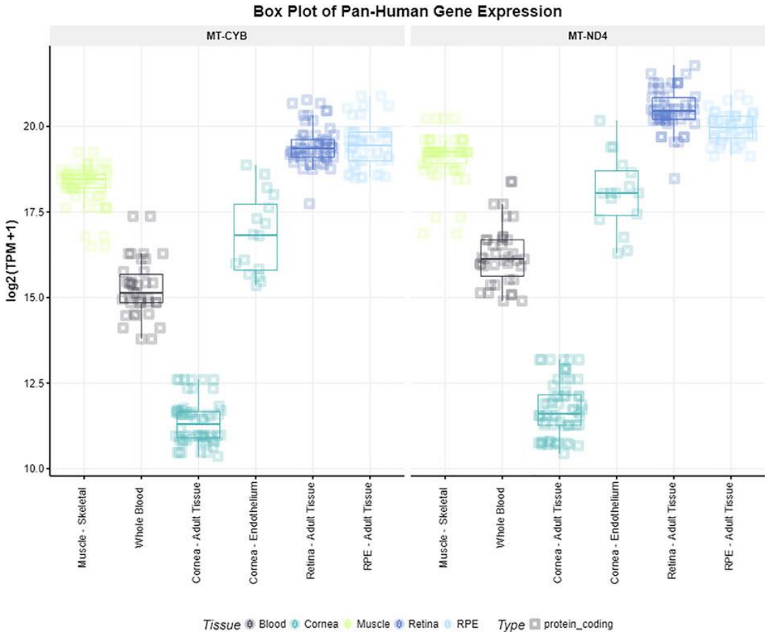
Figure 2. Gene expression levels of the genes MT-CYB and MT-ND4 according to the EyeIntegration database v1.05 for muscle skeletal, whole blood, cornea, retina and RPE tissues.
