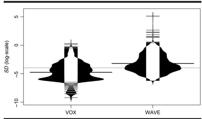
Figure 10. Bean plot visualizing average standard deviations (SDs) of the positional coordinates for both devices during the static tests.
