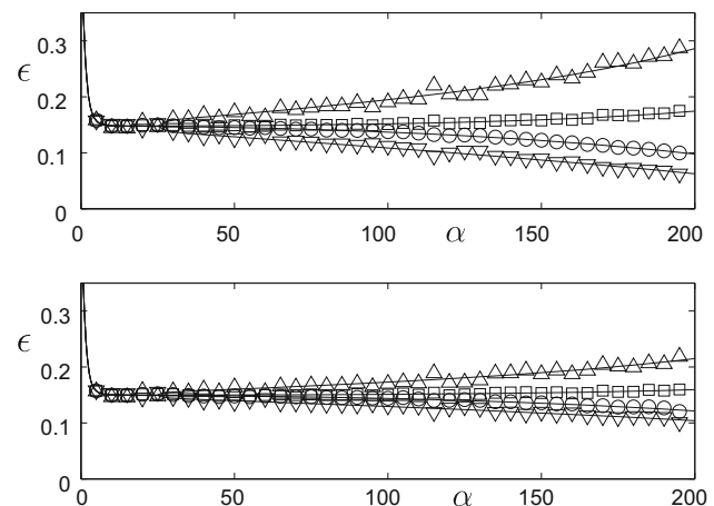
Fig. 1 LVQ1 in the presence of a concept drift with linearly increasing p_1(\alpha) given by \alpha_o = 20, \alpha_{\text{end}} = 200, p_{\max} = 0.8 in (38). Solid lines correspond to the integration of ODE with initialization as in Eq. (37). We set v_{1,2} = 0.4 and \lambda = 1 in the density (4). The upper graph corresponds to LVQ1 without weight decay, the lower graph displays results for \gamma = 0.05 in Eq. (35). In addition, Monte Carlo results for N = 100 are shown: class-wise errors \epsilon^{1,2}(\alpha) are displayed as downward (upward) triangles, respectively; squares mark the reference error \epsilon_{\text{ref}}(\alpha) ; circles correspond to \epsilon_{\text{track}}(\alpha) , cf. Eqs. (30, 31)
