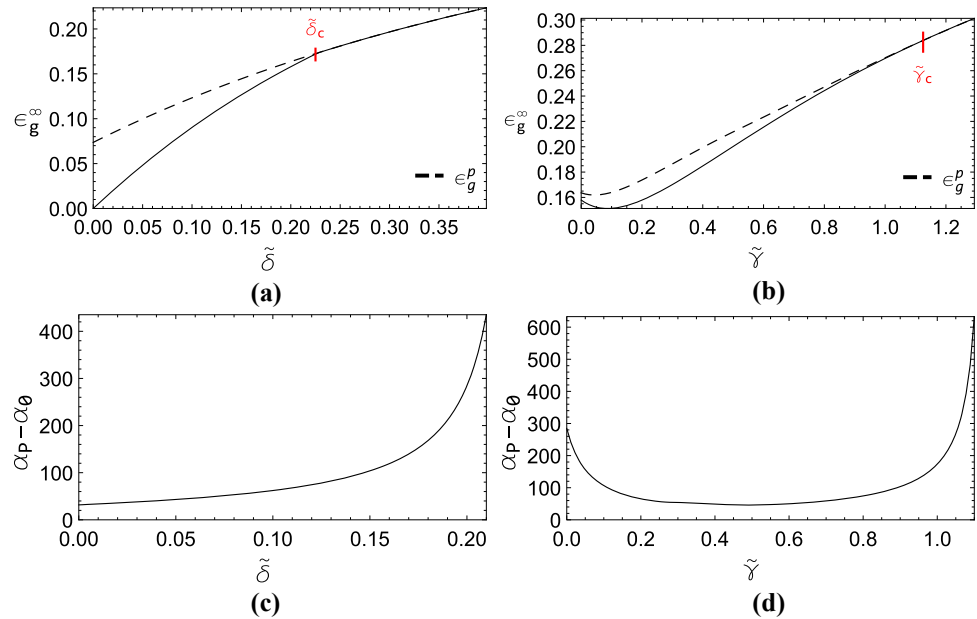
Fig. 6 ReLU-SCM: Generalization error under concept drift in unspecialized plateau states (dashed lines) and final states (solid), as a function of the drift strength (a) and weight decay (b). In (b), \tilde{\delta} = 0.2 . The drift strength \tilde{\delta}_c above which the curves merge is marked in (a) and similar for weight decay \tilde{\gamma}_c in (b). The lower panels show the observed plateau lengths as a function of \tilde{\delta} for \tilde{\gamma} = 0 (c) and as a function of \tilde{\gamma} for fixed \tilde{\delta} = 0.2 (d), respectively
