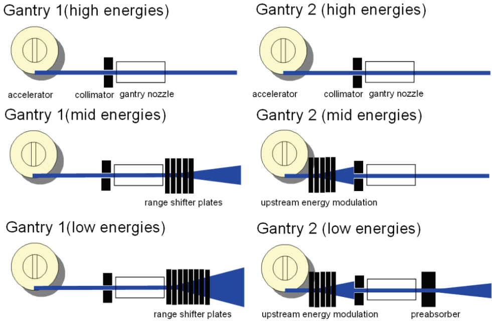
Figure 1. Sketch of the differences in beam-broadening elements between the Gantry 1 and Gantry 2 beam line.
