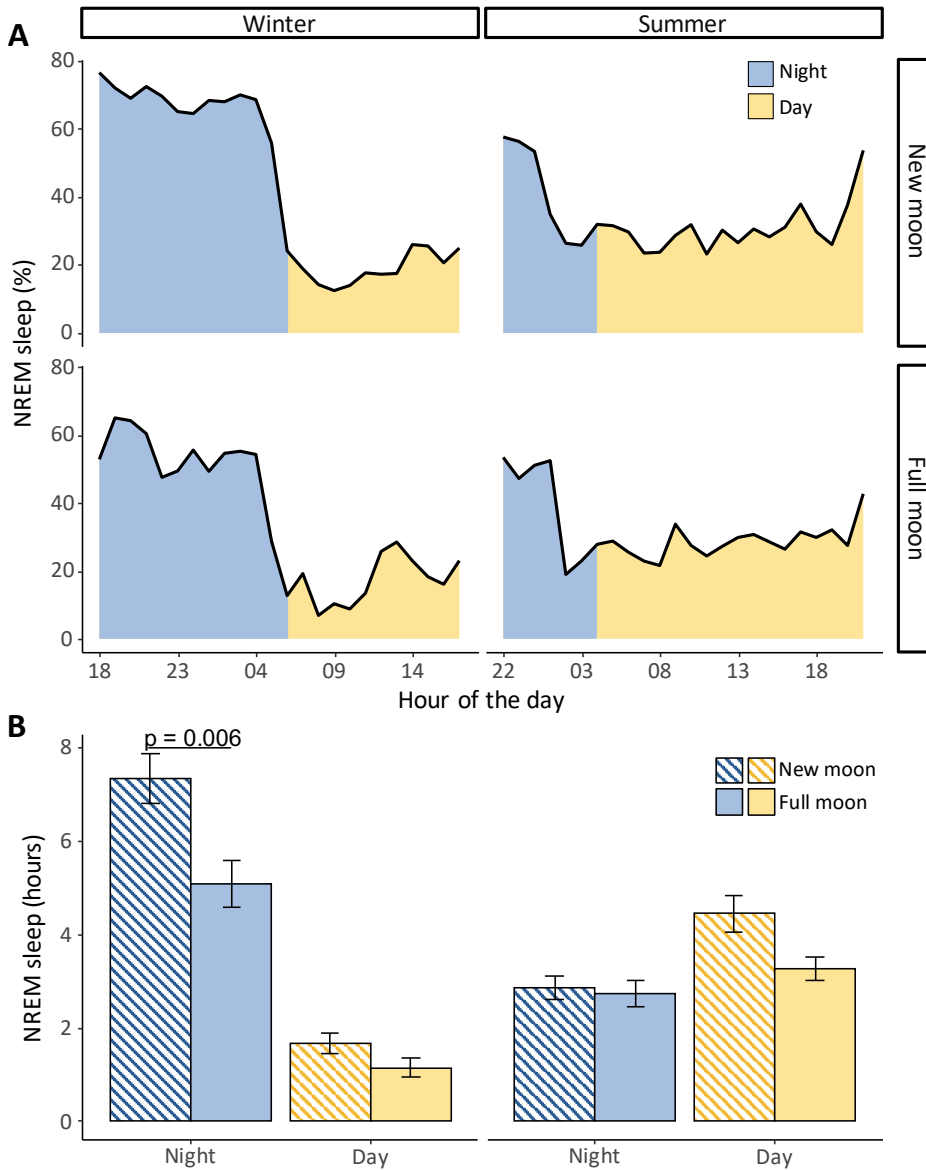
Figure 1. (A) NREM sleep patterns across the day in winter (left) and summer (right) during new moon (top) and full moon (bottom), averaged for all individuals. (B) The effect of moon phase on NREM sleep during the night and day in both winter and summer. During the winter, full moon was associated with a significant reduction of NREM sleep during the night (linear mixed effect model, p = 0.006 ). In both seasons, full moon was associated with a trend towards reduced NREM sleep during daytime (linear mixed effect model, winter: p = 0.052 ; summer: p = 0.053 ).
