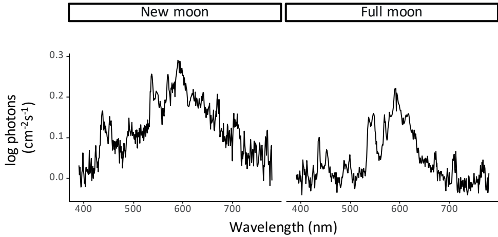
Figure S1. (A) Light spectrum of ALAN reflected by the clouds and perceived by the geese that is derived from the difference between the spectra during clear nights and overcast nights, plotted per moon phase. The relative contribution to the light spectrum that can be attributed to ALAN has a peak around 600 nm and is significantly higher during new moon nights compared to full moon (Figure S1, linear model, p < 0.001 ).
