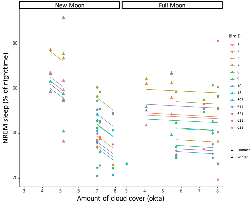
Figure S2. Data based on the model output presented in figure 3C. Cloud cover decreases significantly nightly NREM sleep independent of season (circle: summer; triangles: winter; linear mixed effect model, p < 0.001 ). During full moon, nightly hours of NREM sleep are unaffected by cloud cover increase.
