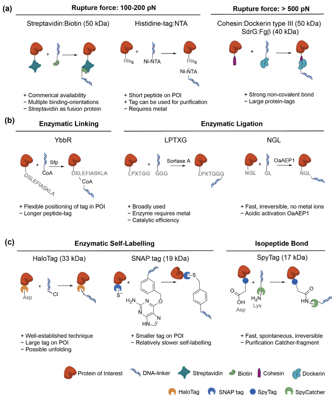
Figure 2. Non-covalent molecular handles and covalent peptide tags for ligation. A comparison of (a) non-covalent conjugation strategies, (b) enzymatic linking and ligation catalyzed by Sfp phosphopantetheinyl transferase, sortase A or the asparaginyl endopeptidase OaAEP1, and (c) enzymatic self-labelling and isopeptide bonds. Amino acid residues are shown in gray and cleaved amino acids are shown in italic.
