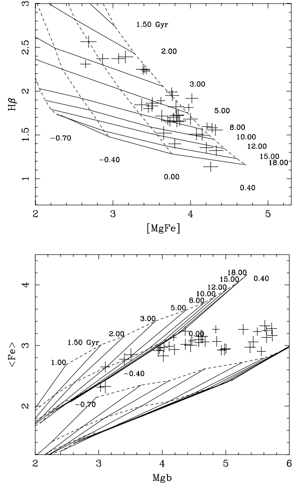
Fig. 3. Line-strength indices measured within the R_e/16 aperture and plotted over BC03 model grids. Note that \langle \text{Fe} \rangle = (\text{Fe}5270 + \text{Fe}5335)/2 and [\text{MgFe}] = (\text{Mgb}(\text{Fe}))^{1/2} . Error bars are 1 standard deviation estimated from the spectrum noise only. Top panel: only the [\text{E}/\text{Fe}] = 0 grid is plotted. Solid lines have constant age while dashed lines have constant metallicity. Age and metallicity values label the corresponding grid lines. Bottom panel: top and bottom grid have [\text{E}/\text{Fe}] = 0 and +0.3 respectively. Grid lines are labelled with the corresponding age and metallicity only for the [\text{E}/\text{Fe}] = 0 grid.
