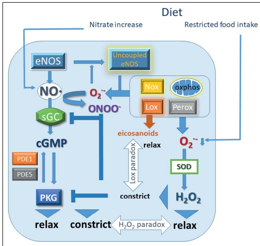
Figure 1. Overview of the nitric oxide (NO)-cyclic guanosine monophosphate signaling cascade and inhibitory oxidative pathways in the vascular wall. cGMP indicates cyclic guanosine monophosphate; eNOS, endothelial nitric oxide synthase; Lox, lipoxygenase; Nox, NADPH oxidase; Oxphos, oxidative phosphorylation; PDE, phosphodiesterase; Perox, peroxidase; PKG, protein kinase G; sGC, soluble guanylyl cyclase; and SOD, superoxide dismutase.
